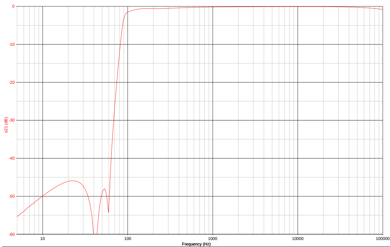
Overall Response (10 dB/div)
