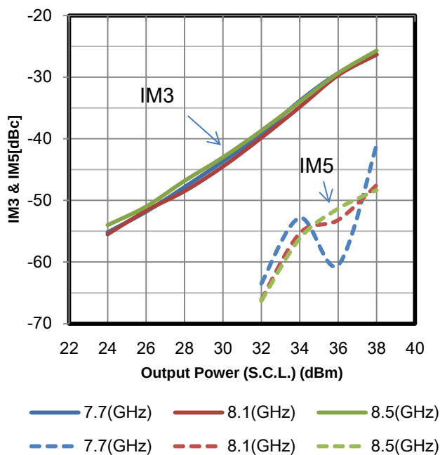
IMD vs. Output Power (S.C.L.) VDS=24V, IDS(DC)=1.75A
