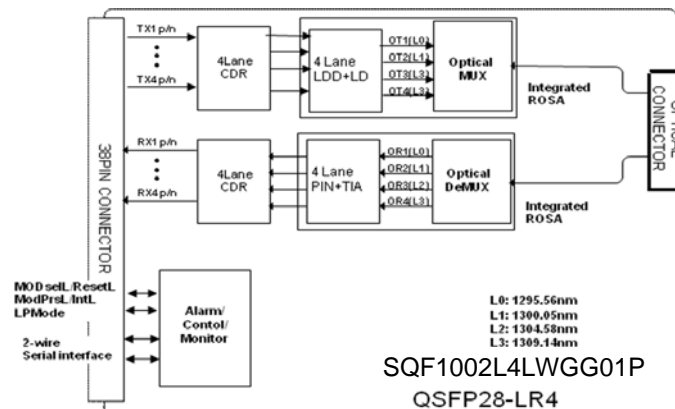
Figure 1.1.: Block Diagram
