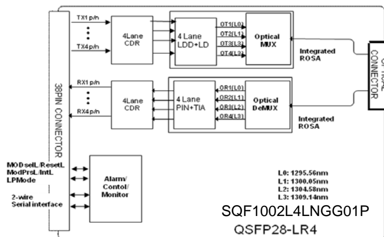
Figure 1.1.: Block Diagram
