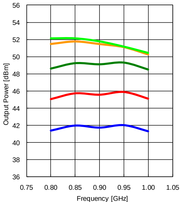
Output Power vs. Frequency V DS =50V I DS(DC) =500mA
