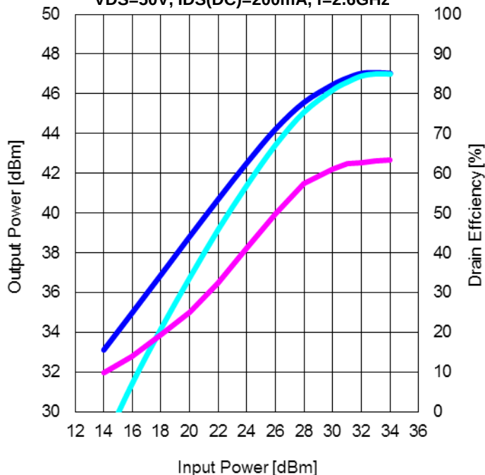
Output Power and Drain Efficiency vs. Input Power VDS=50V, IDS(DC)=200mA, f=2.6GHz
