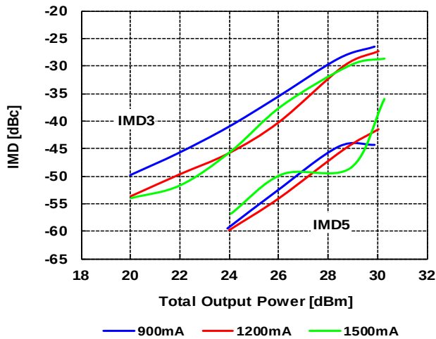
Output Power vs. IMD by Drain Current f=13.75\text{GHz} , V_{DD}=6V , T_c=+25\text{deg.C}
