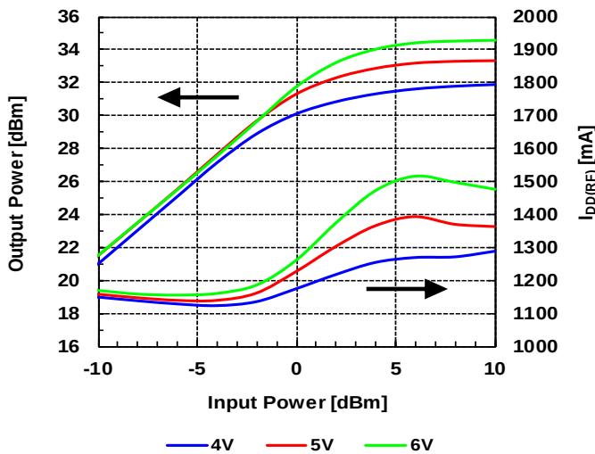
Input Power vs. Output Power by Drain Voltage @13.75GHz, V_{DD}=6.0\text{V} , I_{DD(DC)}=1200\text{mA}
