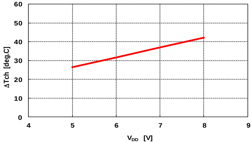
\Delta T_{ch} vs. Drain Voltage (Reference)
