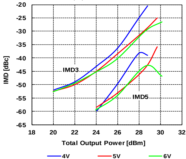
Output Power vs. IMD by Drain Voltage f=14.5\text{GHz} , I_{DD(DC)}=1200\text{mA} , T_c=+25\text{deg.C}
