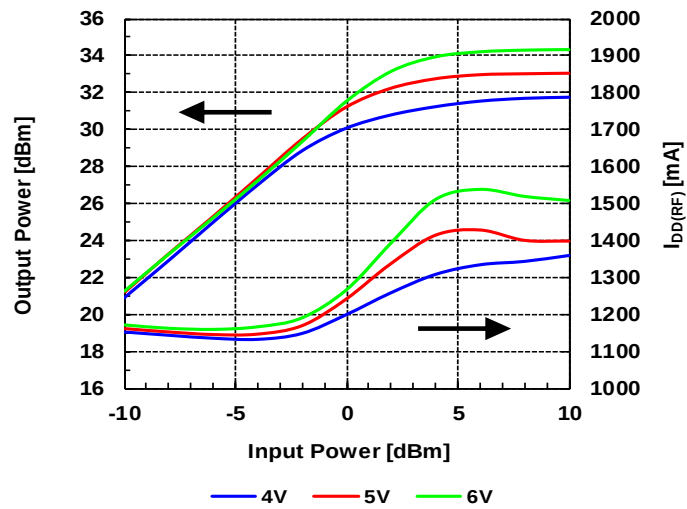
Input Power vs. Output Power by Drain Voltage @14.125GHz, V_{DD}=6.0\text{V} , I_{DD(DC)}=1200\text{mA}
