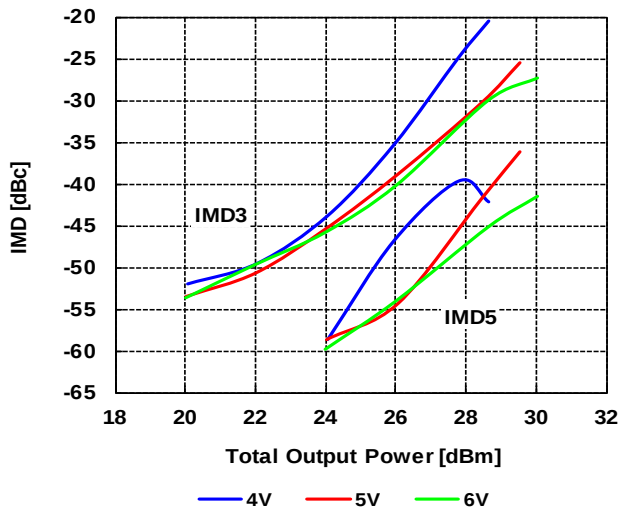
Output Power vs. IMD by Drain Voltage f=13.75\text{GHz} , I_{DD(DC)}=1200\text{mA} , T_c=+25\text{deg.C}
