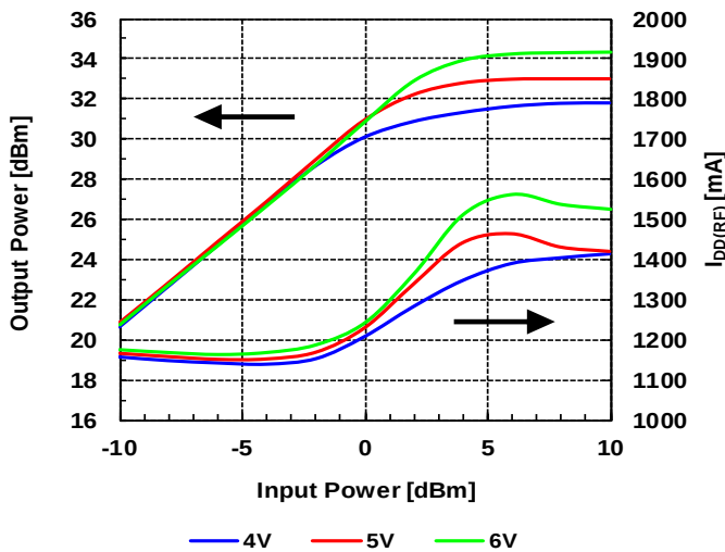
Input Power vs. Output Power by Drain Voltage @14.5GHz, V_{DD}=6.0\text{V} , I_{DD(DC)}=1200\text{mA}
