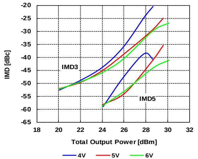
Output Power vs. IMD by Drain Voltage f=14.125\text{GHz} , I_{DD(DC)}=1200\text{mA} , T_c=+25\text{deg.C}
