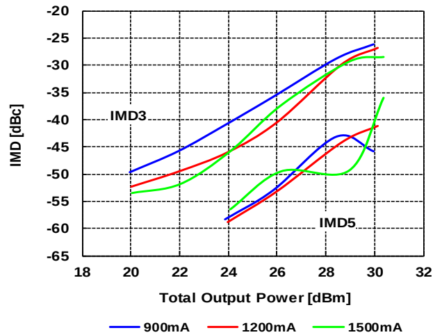
Output Power vs. IMD by Drain Current f=14.125\text{GHz} , V_{DD}=6V , T_c=+25\text{deg.C}
