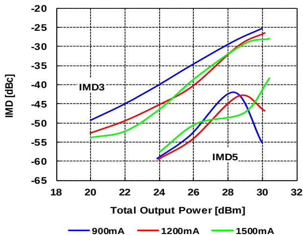
Output Power vs. IMD by Drain Current f=14.5\text{GHz} , V_{DD}=6V , T_c=+25\text{deg.C}
