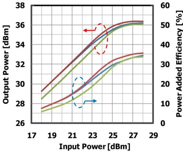
Input Power vs. Output Power, Power Added Efficiency by Temperature VDS=10V @8.5GHz
