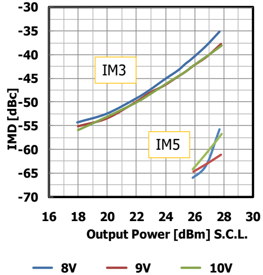
IMD Performance vs. Output Power by Drain Voltage IDS(DC)=1100mA @7.5GHz
