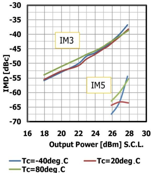
IMD Performance vs. Output Power by Temperature VDS=10V @7.9GHz
