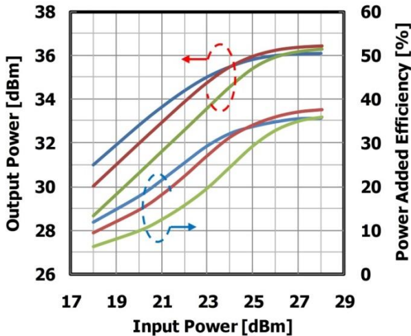
Input Power vs. Output Power, Power Added Efficiency by Temperature VDS=10V @7.9GHz
