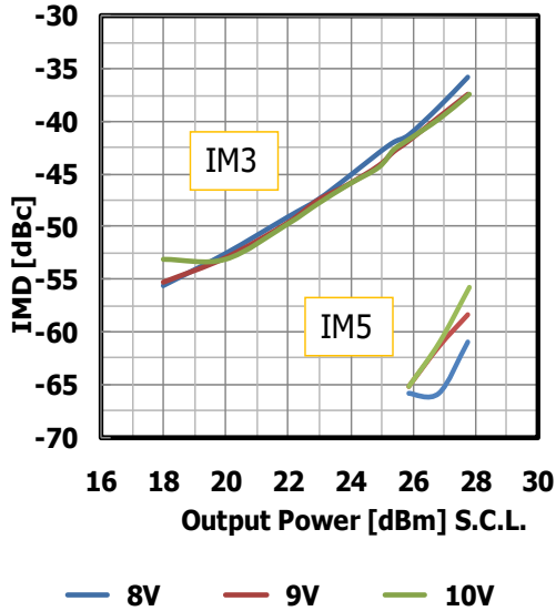
IMD Performance vs. Output Power by Drain Voltage IDS(DC)=1100mA @7.9GHz
