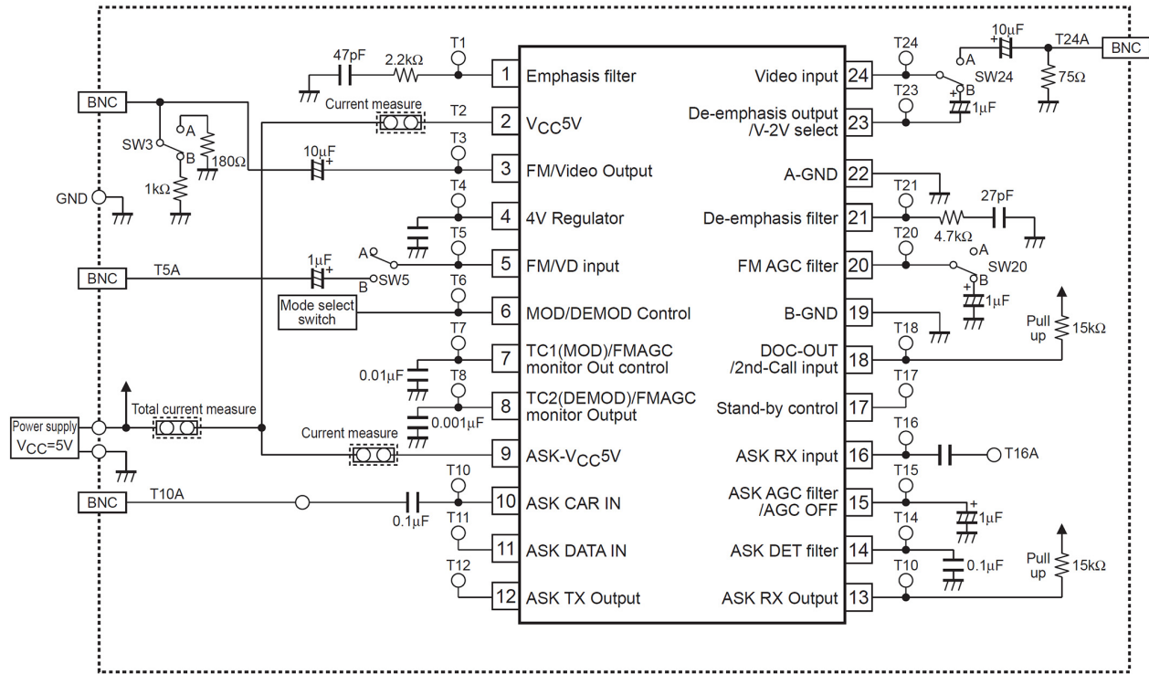
Figure 4. Test Circuit
