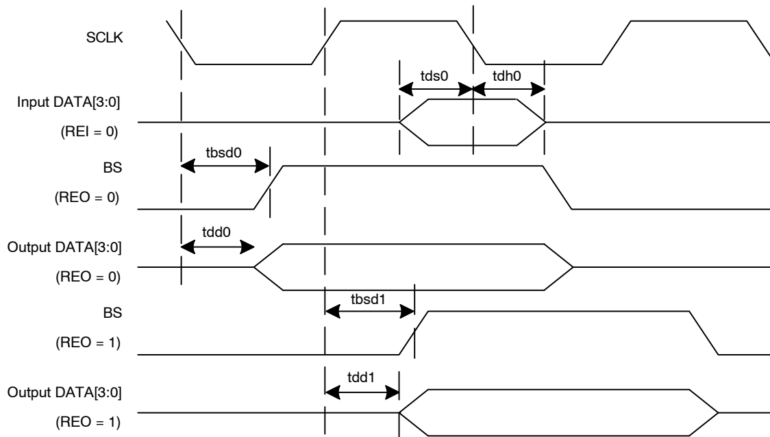
Figure 23. Parallel Interface
