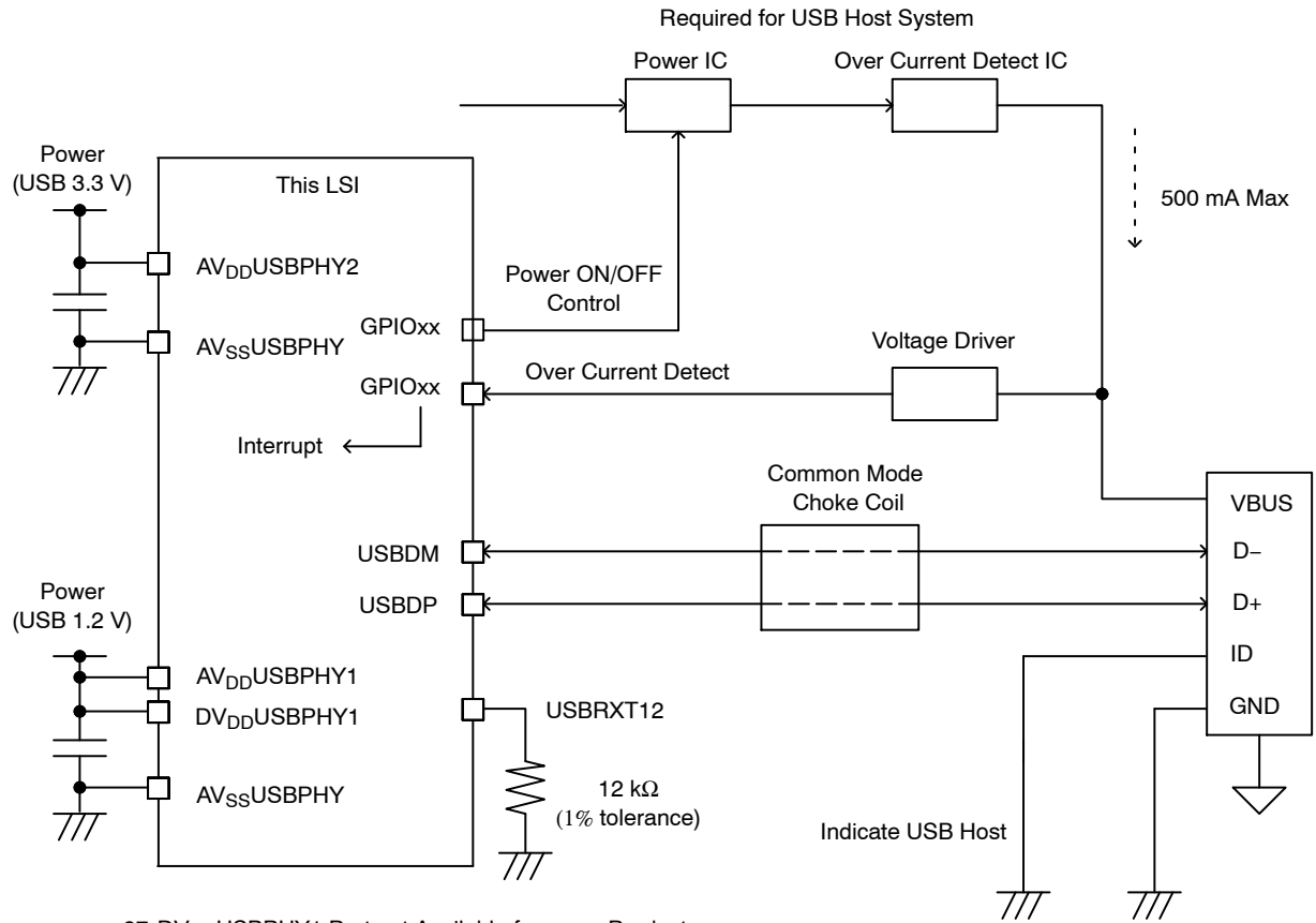
Figure 45. USB Host
