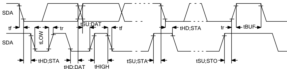
Figure 14. AC Characteristics – I^2C
