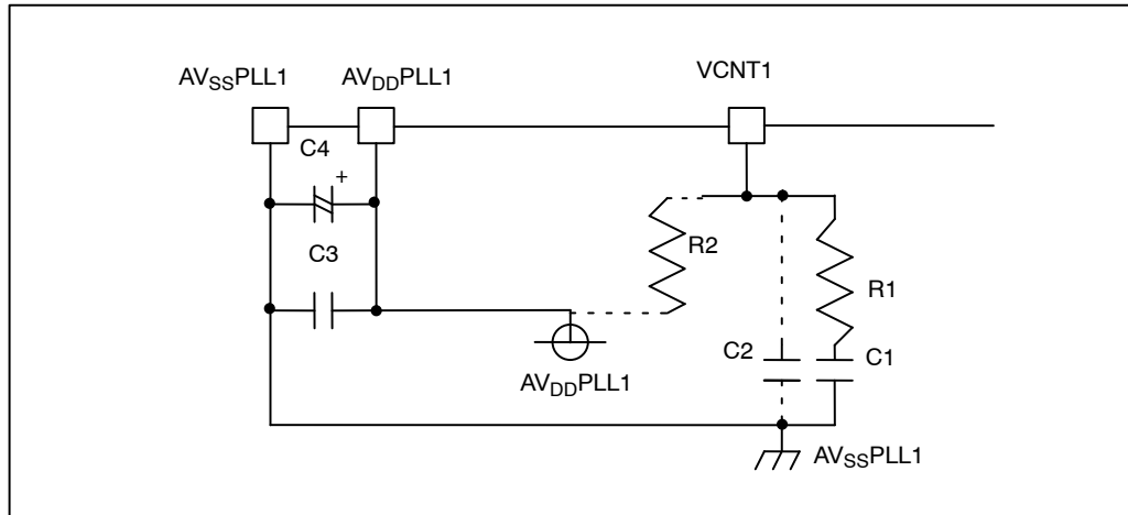
Figure 40. PLL1 (System)
