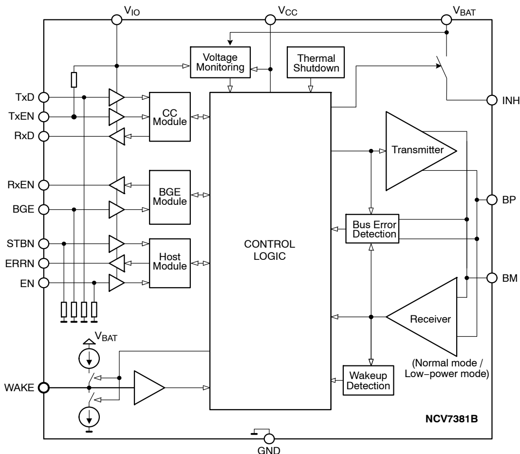
Figure 1. Block Diagram
