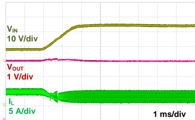
Figure 29. Line Transient Response (8 V - 24 V, I OUT = 2 A)
