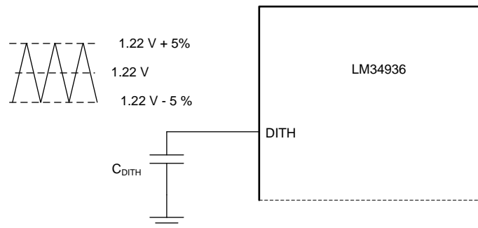
Figure 24. Dither Operation
