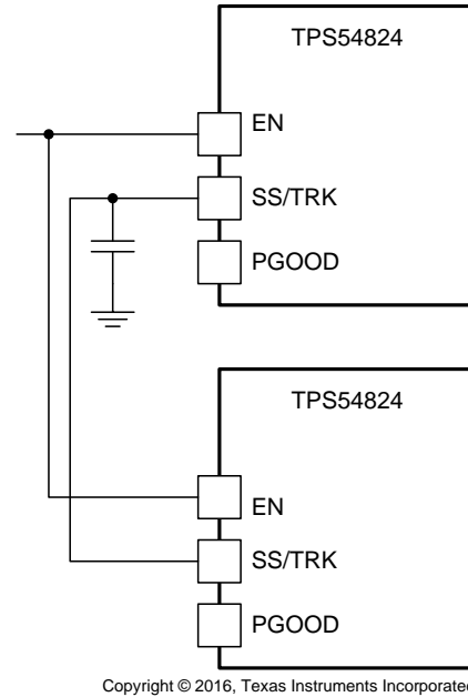
图 26. Ratiometric Start-Up Sequence
