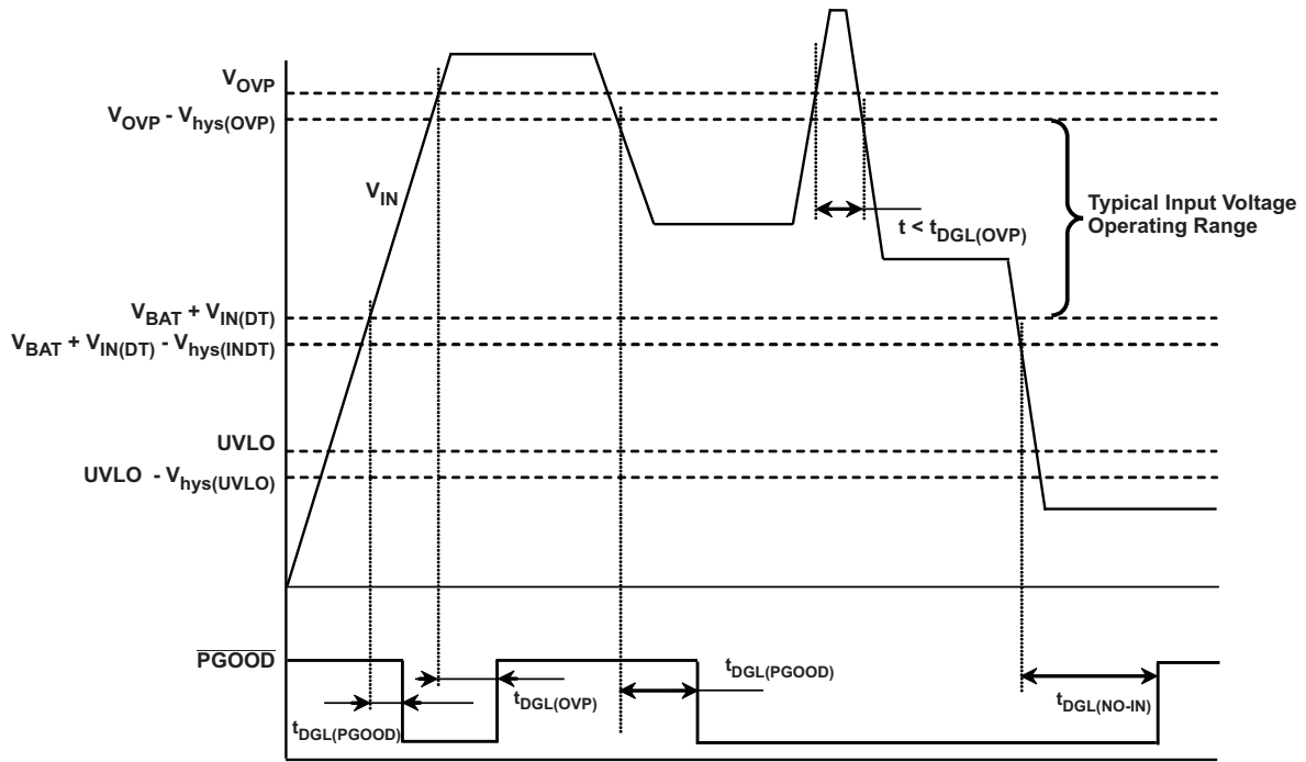
图 1. Power-Up, Power-Down, Power Good Indication
