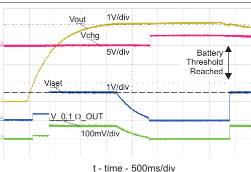
图 25. Battery Removal with OUT and TS Disconnect 1st, With 100 \Omega Load
