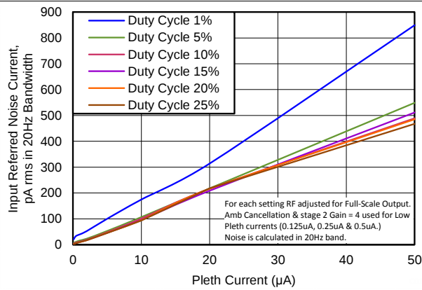
Figure 17. Input-Referred Noise Current vs PLETH Current (BW = 20 Hz, PRF = 600 Hz)
