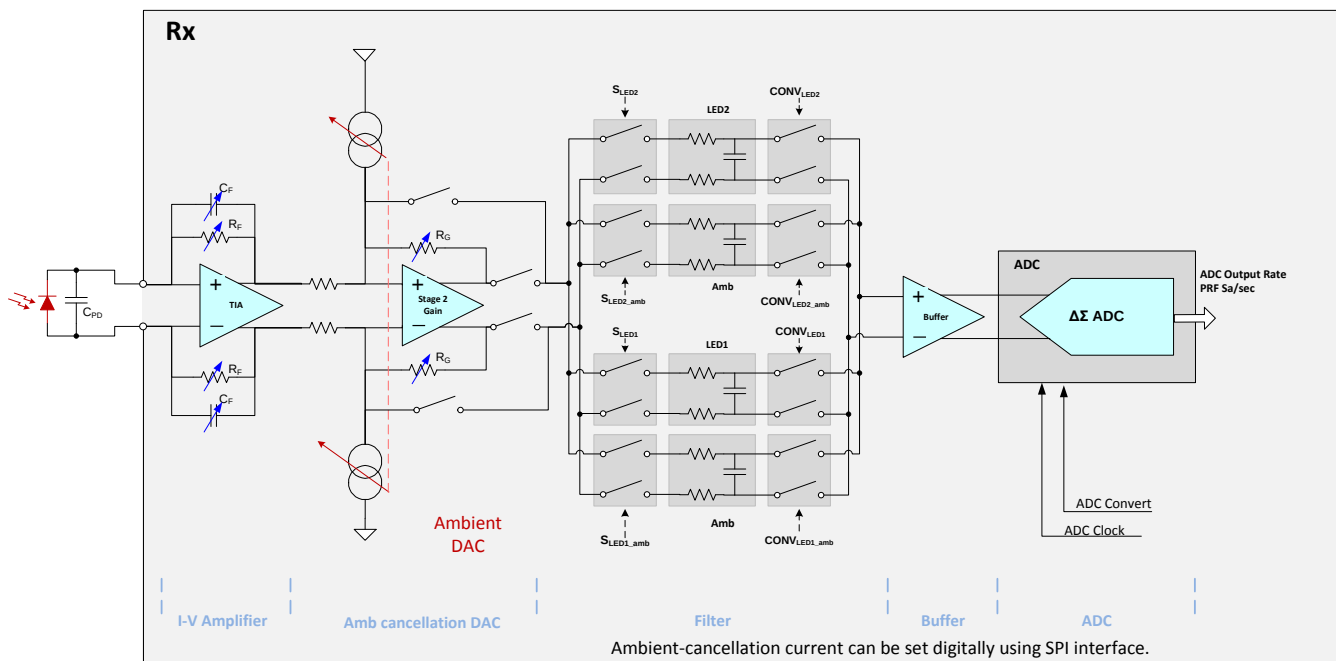
Figure 55. Receiver Front-End
