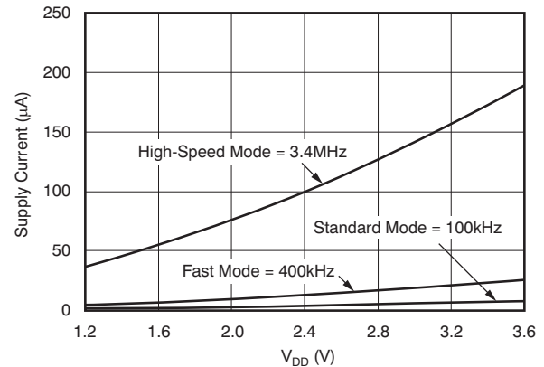
Figure 7. Supply Current (Part Not Addressed) vs Supply Voltage
