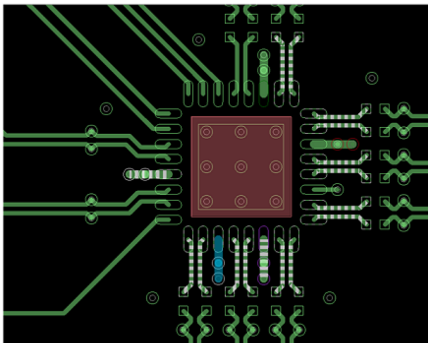
Figure 47. Example Layout
