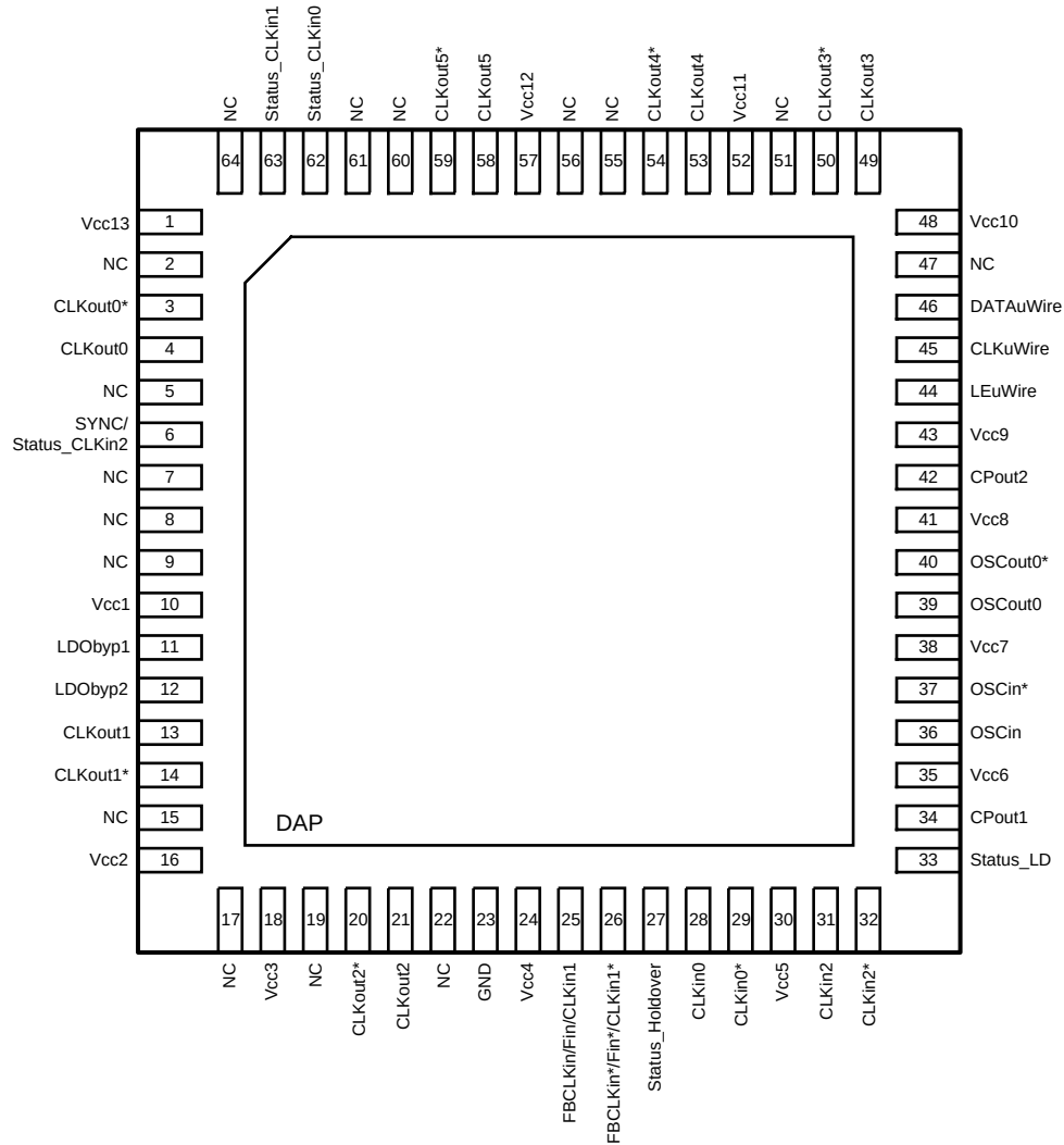
Pin Functions
