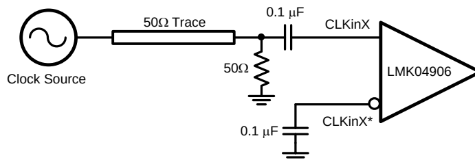
Figure 24. CLKInX/CLKInX* Single-Ended Termination
