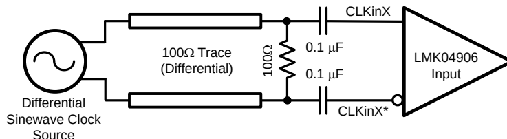
Figure 23. CLKInX/CLKInX* Termination for a Differential Sinewave Reference Clock Source
