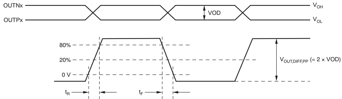
Figure 1. Output Voltage and Rise/Fall Time
