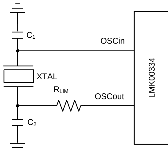
Figure 18. Crystal Interface
