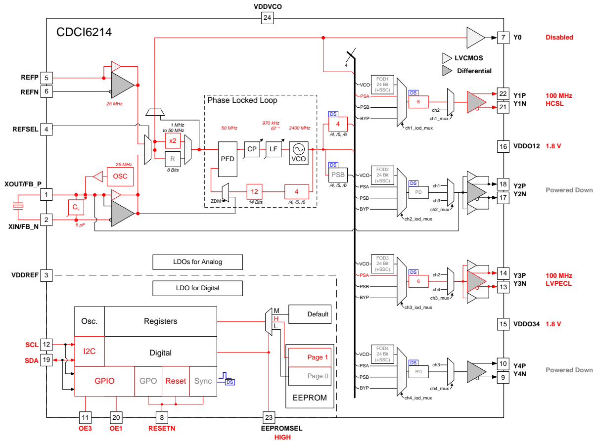
Figure 32. CDCI6214 - Pre-Configured EEPROM Page 0
