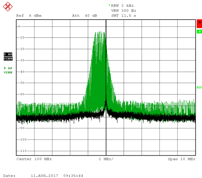
Figure 23. 100 MHz With 0.5% Spread Spectrum (Trace 3) and Without (Trace 2)
