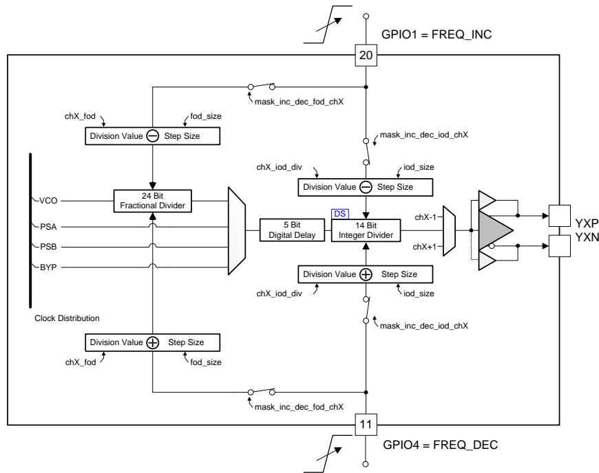
图 25. Frequency Increment and Decrement by Control Pin
