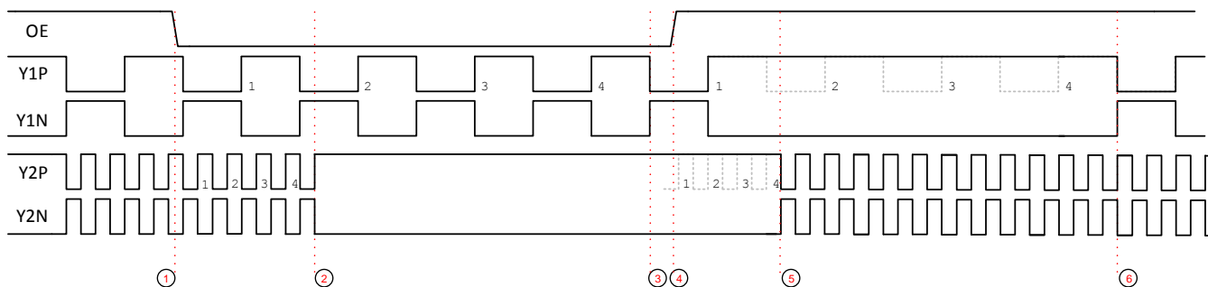
图 26. Individual Output Enable and Disable
