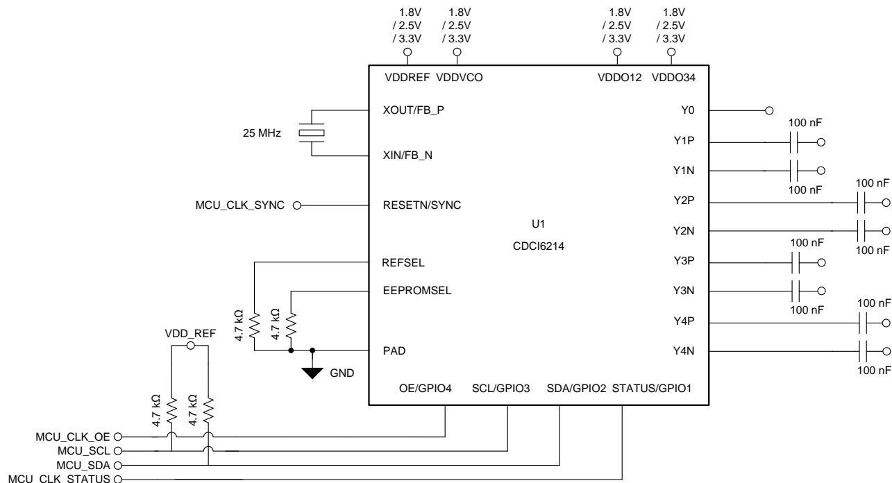
Figure 90. Typical Serial Interface Application Schematic
