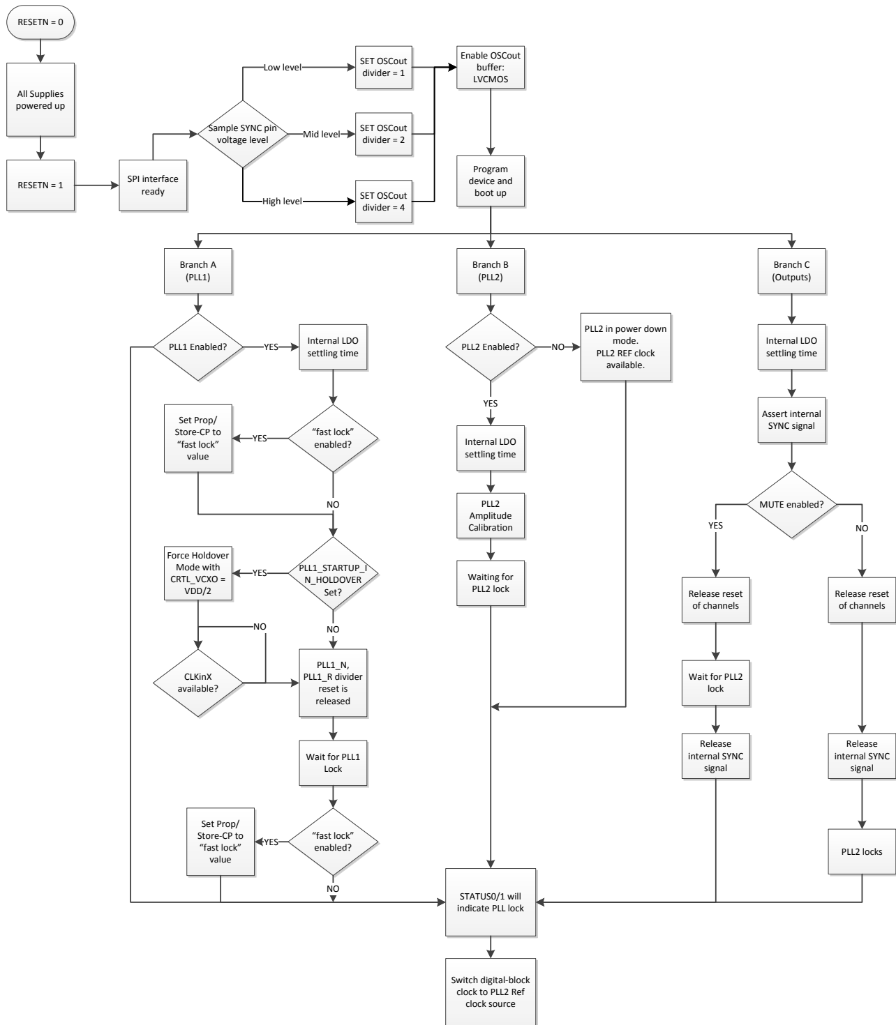
Figure 50. Detailed Power-Up Sequence
