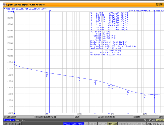
Figure 8. LMK0461x CLKout2 Phase Noise VCO Frequency = 5898.24 MHz CLKout2 Frequency = 1966.08 MHz HSDS 8 mA
