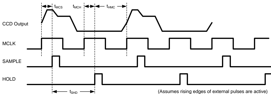
Figure 13. SH3 Timing Mode – ADC Rate Clock Input
