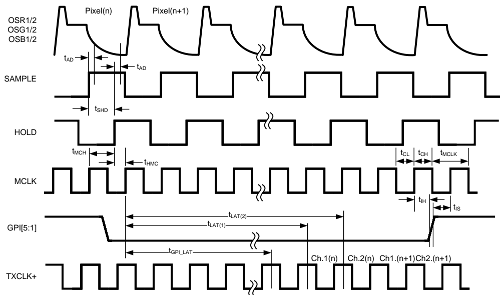
Above timing relationships between SAMPLE, HOLD and MCLK are for AFEPHASE = 11. For other AFEPHASE settings, the sampling timing can move earlier by ¼, ½ or ¾ pixel period with respect to MCLK, but the latency as shown above will remain constant.
