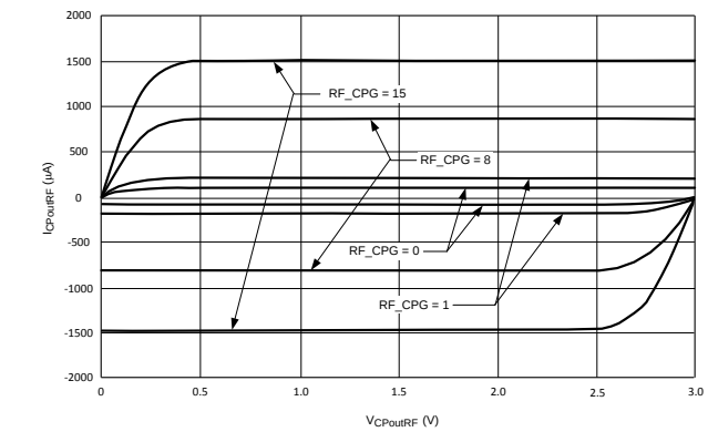
Figure 14. RF PLL Charge Pump Current
