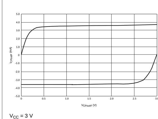
Figure 15. IF PLL Charge Pump Current
