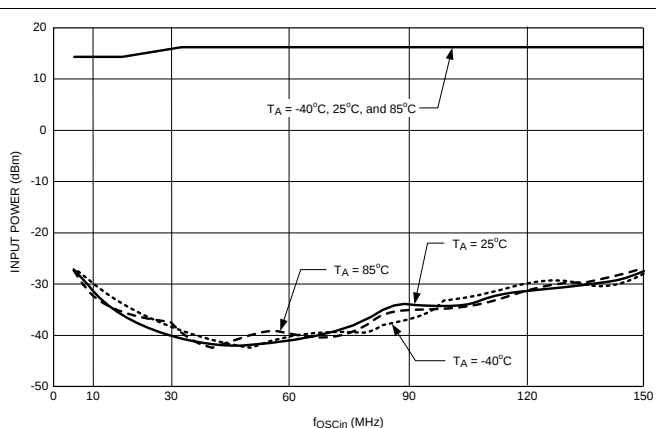
Figure 7. OSCin Sensitivity
