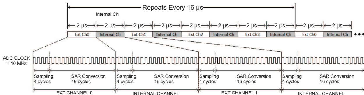
Figure 5-20. ADC Clock Timing Diagram
