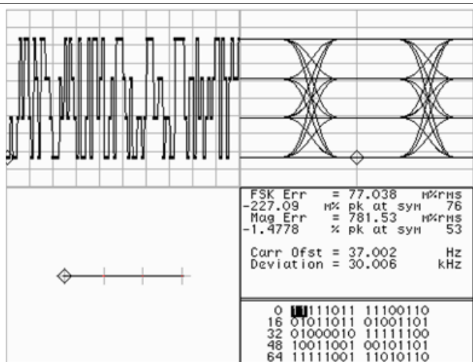
Figure 70. 4FSK Modulation Quality
