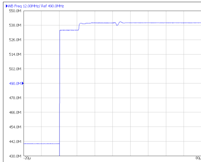
Figure 79. External VCO to Internal VCO Switching
