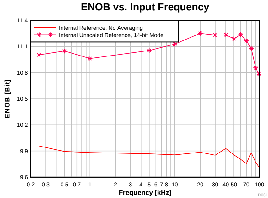
图 5-24. ENOB vs. Input Frequency
