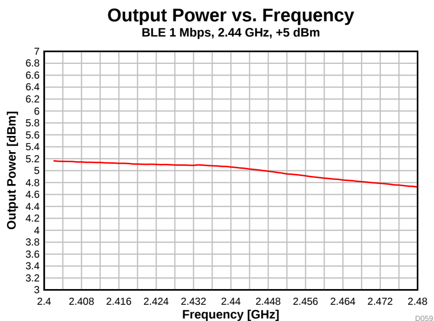
图 5-23. Output Power vs. Frequency (BLE 1 Mbps, 2.44 GHz, +5 dBm)
