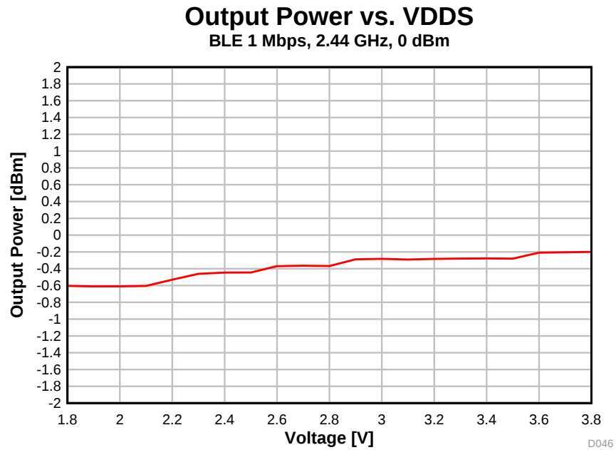
图 5-20. Output Power vs. Supply Voltage (VDDS) (BLE 1 Mbps, 2.44 GHz)
