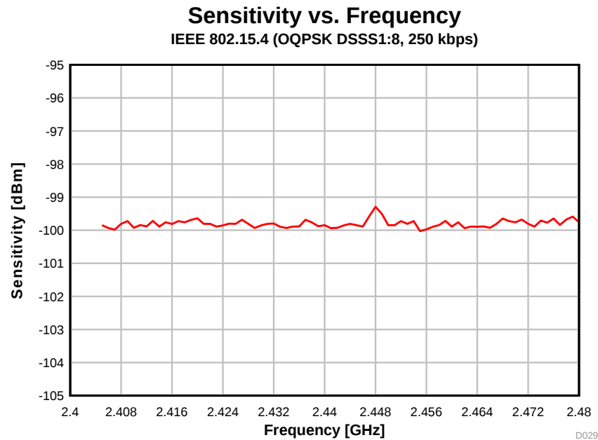
图 5-12. Sensitivity vs. Frequency (250 kbps, 2.44 GHz)
