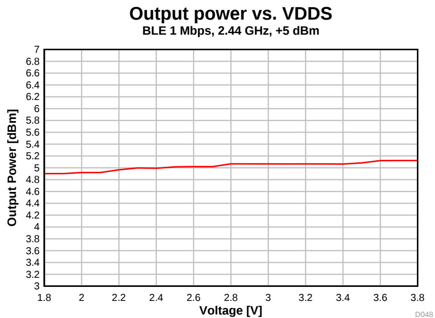
图 5-21. Output Power vs. Supply Voltage (VDDS) (BLE 1 Mbps, 2.44 GHz, +5 dBm)
