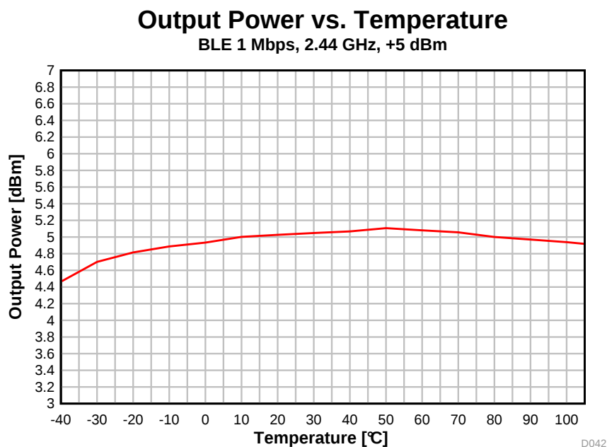
图 5-19. Output Power vs. Temperature (BLE 1 Mbps, 2.44 GHz, +5 dBm)
