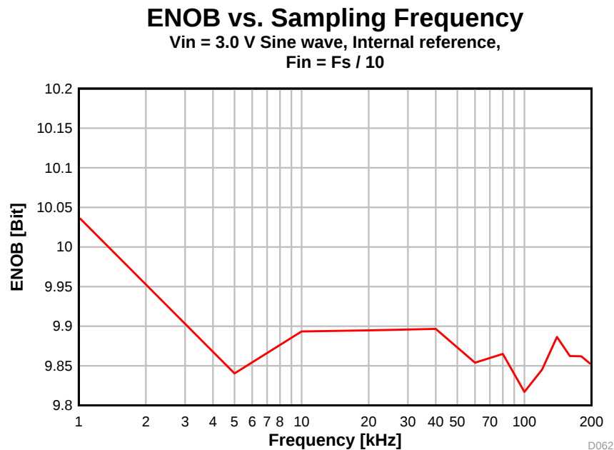
图 5-25. ENOB vs. Sampling Frequency
