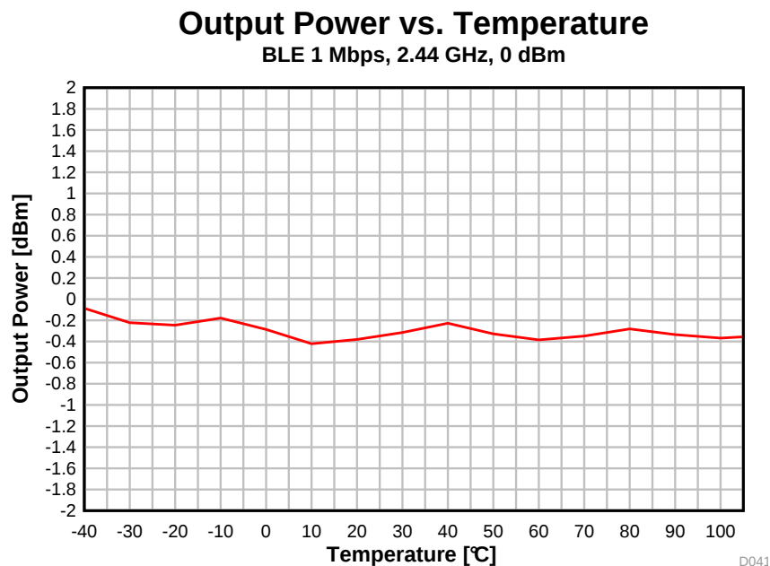
图 5-18. Output Power vs. Temperature (BLE 1 Mbps, 2.44 GHz)
