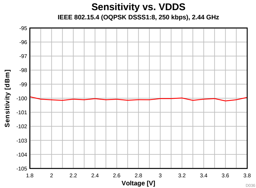
图 5-17. Sensitivity vs. Supply Voltage (VDD5) (250 kbps, 2.44 GHz)
