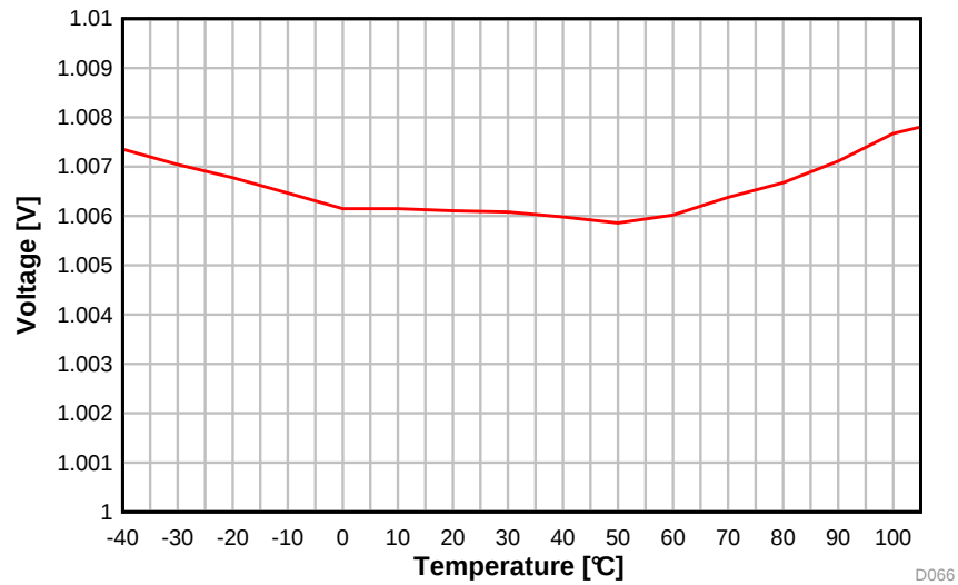
图 5-28. ADC Accuracy vs. Temperature
