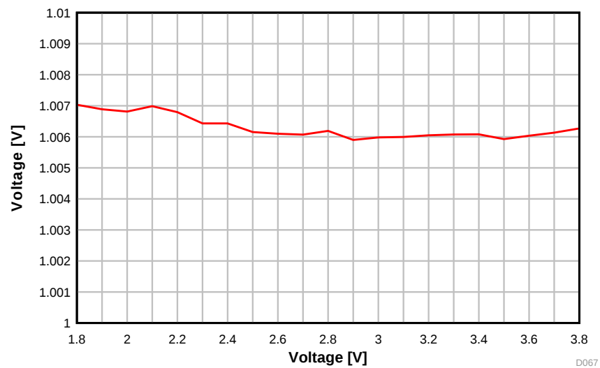
图 5-29. ADC Accuracy vs. Supply Voltage (VDDS)
