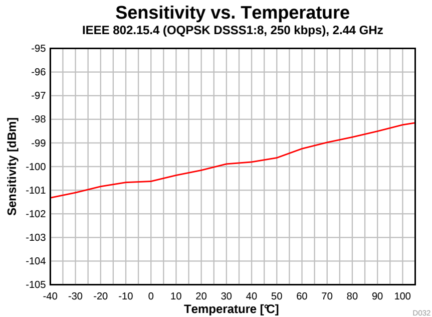
图 5-14. Sensitivity vs. Temperature (250 kbps, 2.44 GHz)
