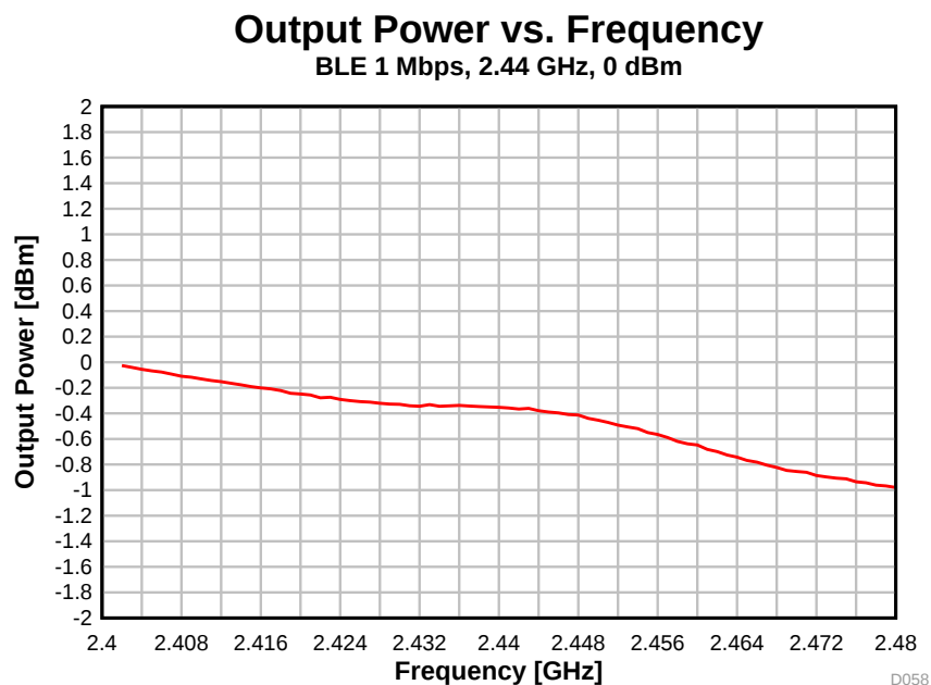
图 5-22. Output Power vs. Frequency (BLE 1 Mbps, 2.44 GHz)
