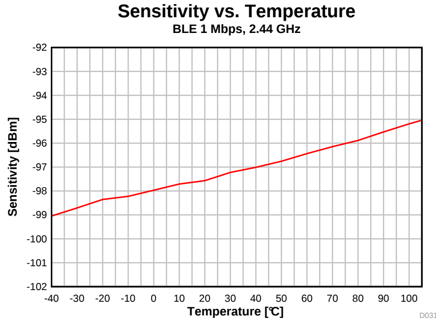
图 5-13. Sensitivity vs. Temperature (BLE 1 Mbps, 2.44 GHz)
