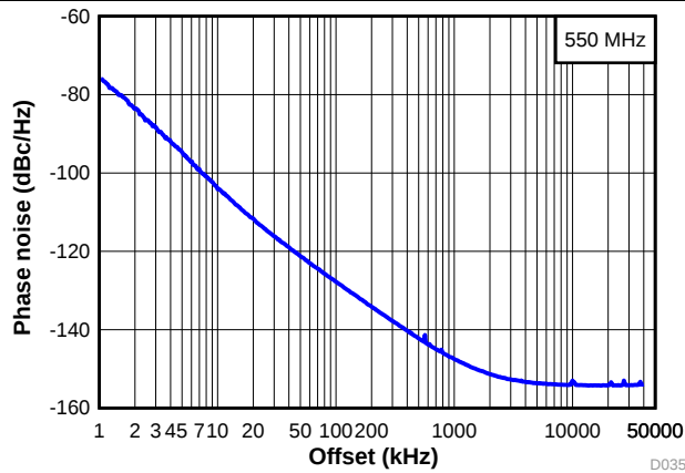
图 5. Open-Loop VCO Phase Noise at 550 MHz
