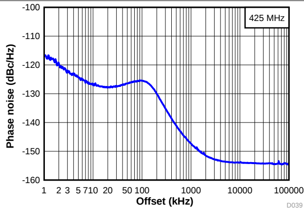
图 9. Wide Band Phase Noise at 425 MHz
