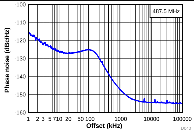
图 10. Wide Band Phase Noise at 487.5 MHz
