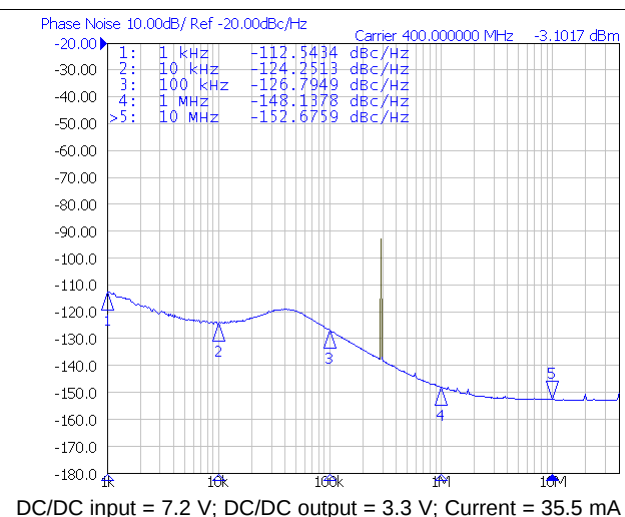
图 176. Phase Noise With DC/DC Power Supply
