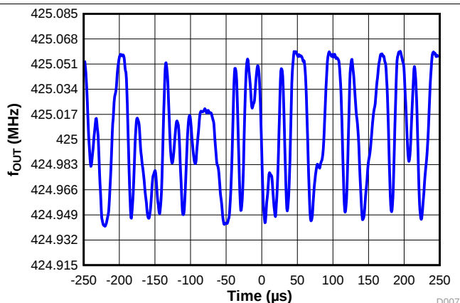
图 19. 4-Level GFSK Modulation
