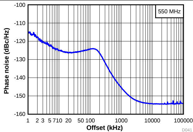
图 11. Wide Band Phase Noise at 550 MHz
