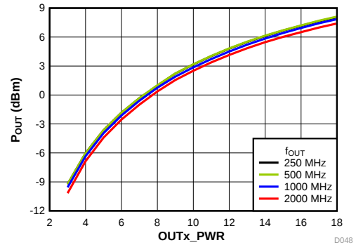
图 156. Output Power vs Power Control Bits
