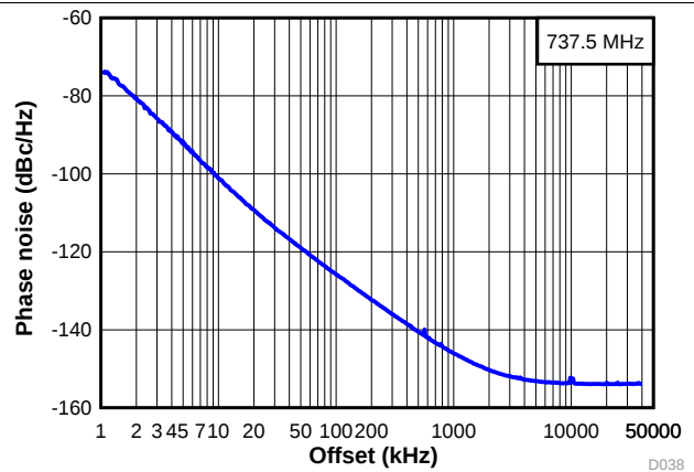
图 8. Open-Loop VCO Phase Noise at 737.5 MHz
