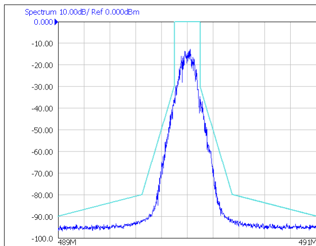
图 171. Gaussian 4FSK Modulated Spectrum
