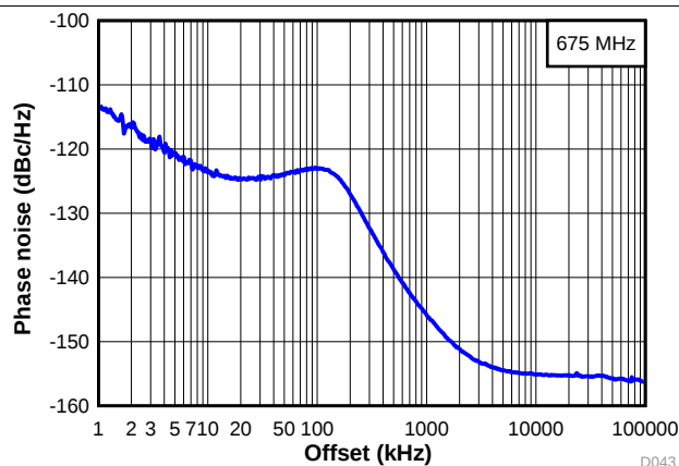
图 13. Wide Band Phase Noise at 675 MHz
