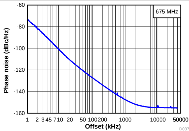
图 7. Open-Loop VCO Phase Noise at 675 MHz
