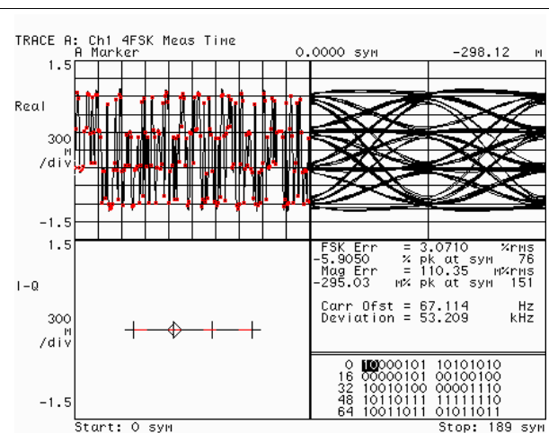
图 172. Gaussian 4FSK Modulation Quality
