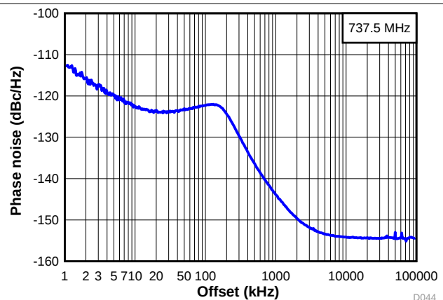
图 14. Wide Band Phase Noise at 737.5 MHz
