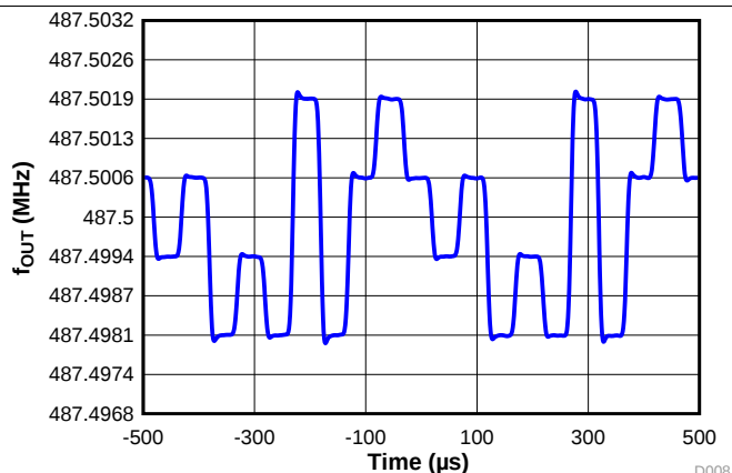
图 20. Discrete-Level FSK Modulation
