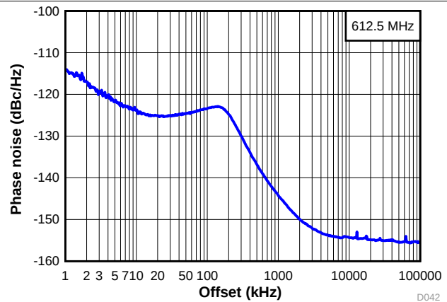
图 12. Wide Band Phase Noise at 612.5 MHz
