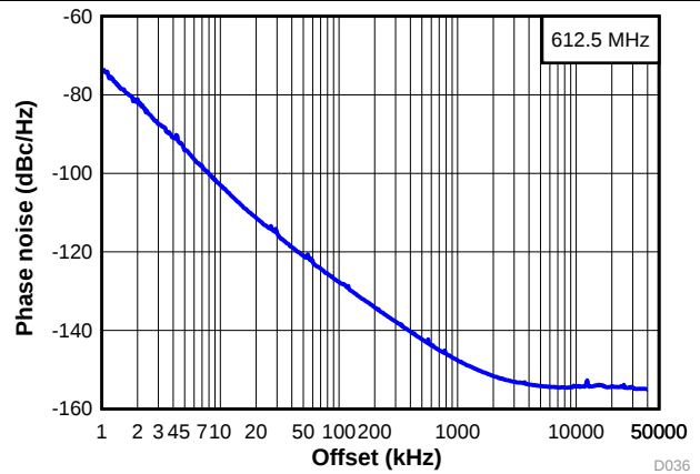
图 6. Open-Loop VCO Phase Noise at 612.5 MHz
