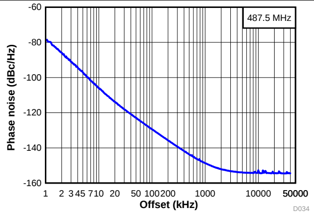
图 4. Open-Loop VCO Phase Noise at 487.5 MHz
