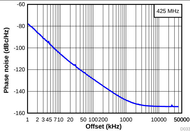
图 3. Open-Loop VCO Phase Noise at 425 MHz
