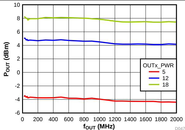
图 17. Output Power vs Frequency
