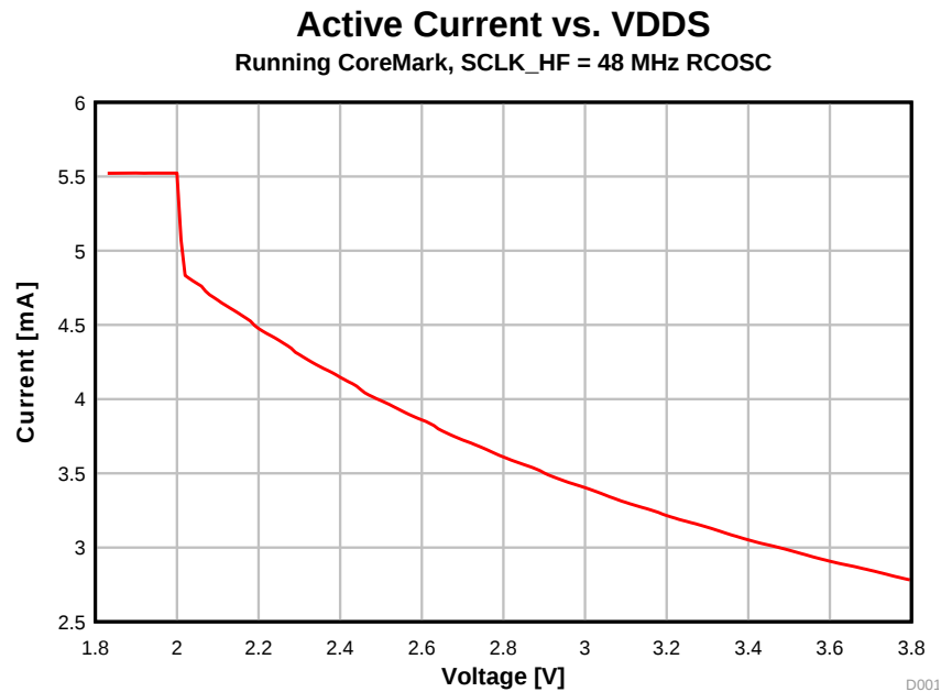
图 5-4. Active Mode (MCU) Current vs. Supply Voltage (VDD)
