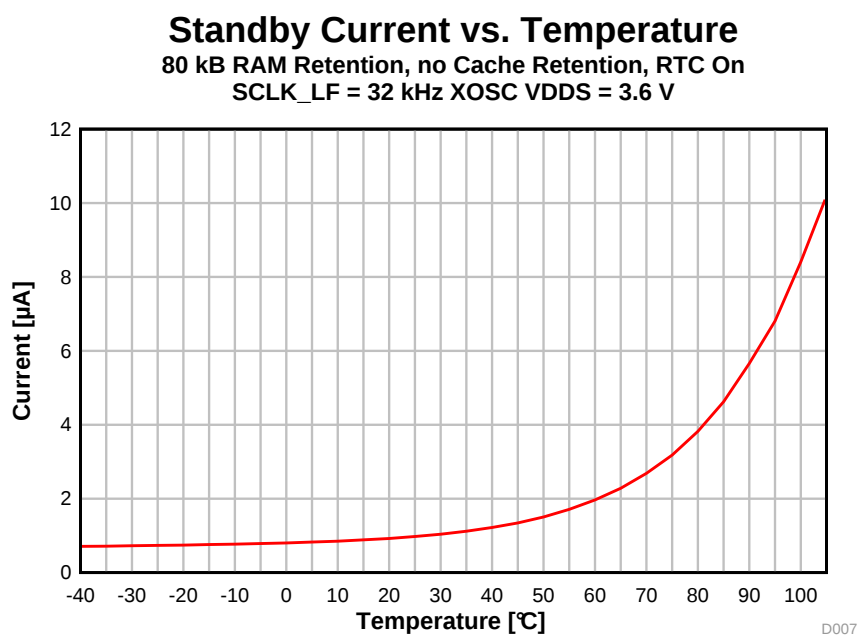
图 5-6. Standby Mode (MCU) Current vs. Temperature (VDD5 = 3.6 V)
