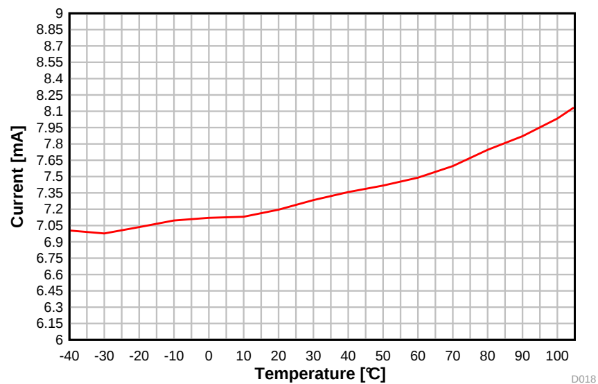
图 5-14. TX Current vs. Temperature (BLE 1 Mbps, 2.44 GHz)
