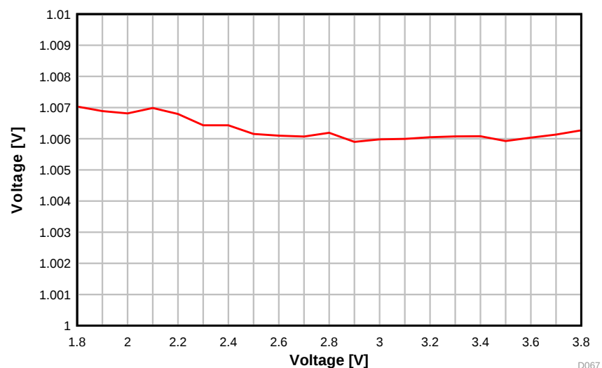
图 5-44. ADC Accuracy vs. Supply Voltage (VDDS)
