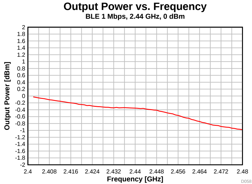
图 5-37. Output Power vs. Frequency (BLE 1 Mbps, 2.44 GHz)
