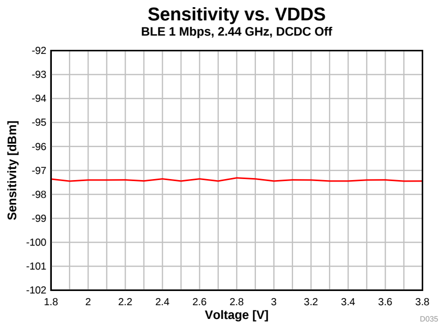
图 5-26. Sensitivity vs. Supply Voltage (VDD) (BLE 1 Mbps, 2.44 GHz, DCDC Off)
