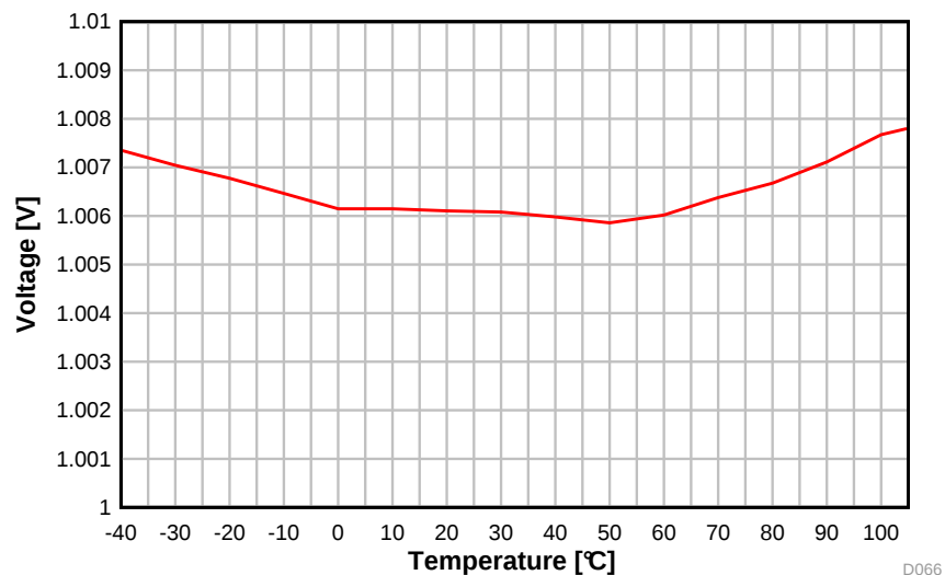
图 5-43. ADC Accuracy vs. Temperature
