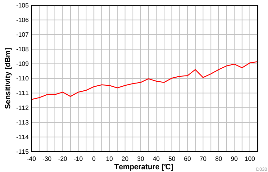
图 5-21. Sensitivity vs. Temperature (50 kbps, 868.3 MHz)
