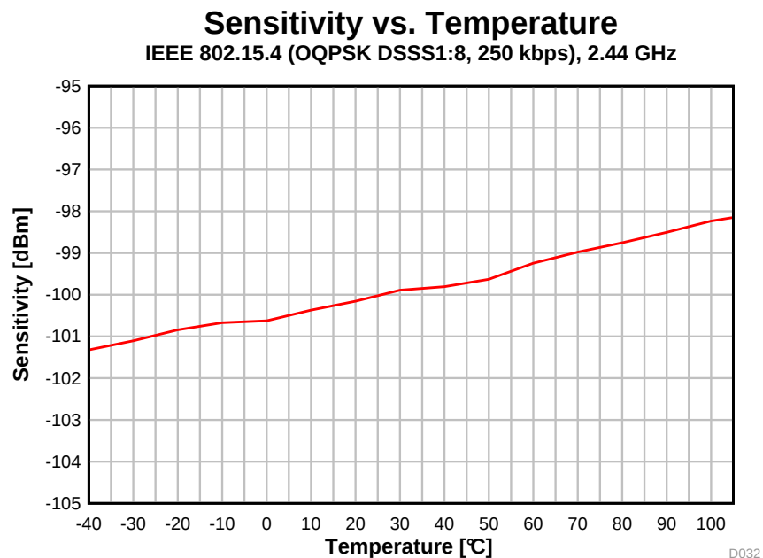
图 5-23. Sensitivity vs. Temperature (250 kbps, 2.44 GHz)
