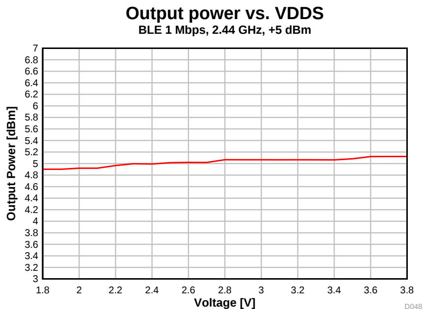
图 5-34. Output Power vs. Supply Voltage (VDDS) (BLE 1 Mbps, 2.44 GHz, +5 dBm)
