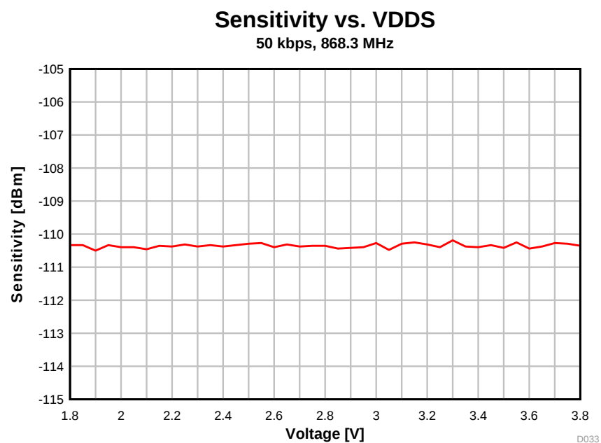
图 5-24. Sensitivity vs. Supply Voltage (VDDDS) (50 kbps, 868.3 MHz)
