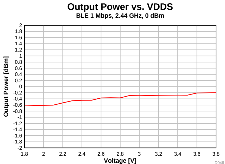
图 5-33. Output Power vs. Supply Voltage (VDDS) (BLE 1 Mbps, 2.44 GHz)
