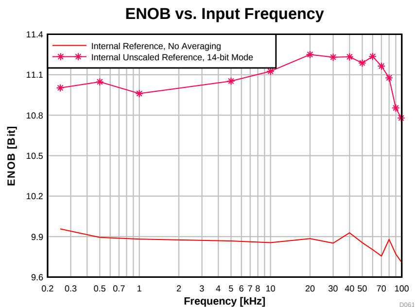
图 5-39. ENOB vs. Input Frequency
