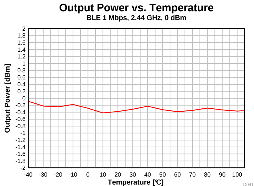
图 5-30. Output Power vs. Temperature (BLE 1 Mbps, 2.44 GHz)
