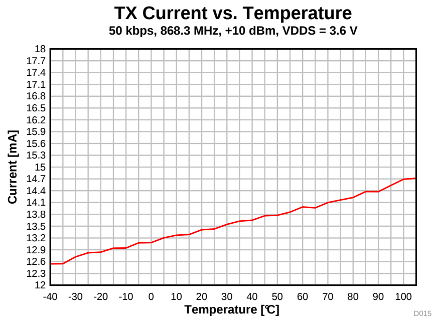
图 5-13. TX Current vs. Temperature (50 kbps, 868.3 MHz, VDD S = 3.6 V)
