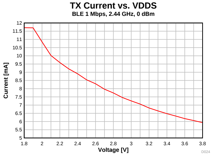
图 5-16. TX Current vs. Supply Voltage (VDD5) (BLE 1 Mbps, 2.44 GHz)
