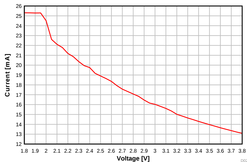
图 5-15. TX Current vs. Supply Voltage (VDD5) (50 kbps, 868.3 MHz)
