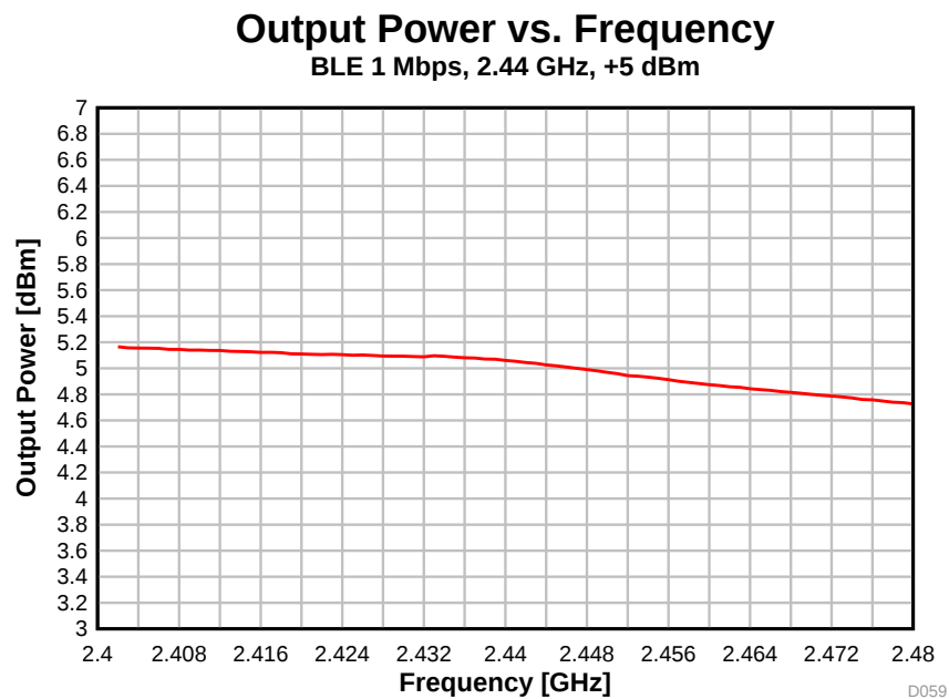
图 5-38. Output Power vs. Frequency (BLE 1 Mbps, 2.44 GHz, +5 dBm)
