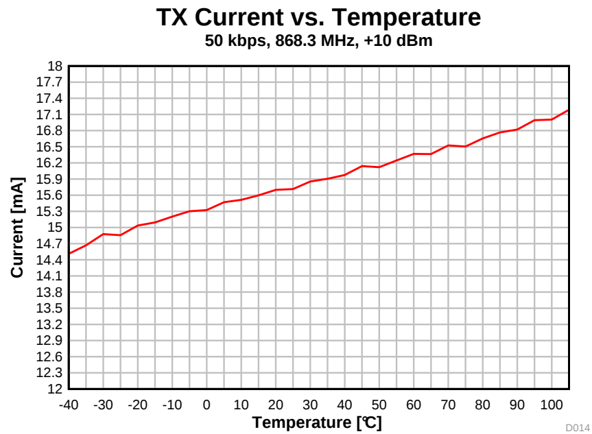
图 5-12. TX Current vs. Temperature (50 kbps, 868.3 MHz)
