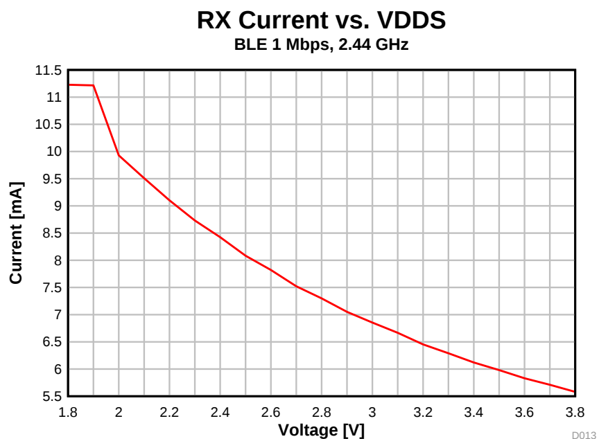
图 5-11. RX Current vs. Supply Voltage (VDDS) (BLE 1 Mbps, 2.44 GHz)
