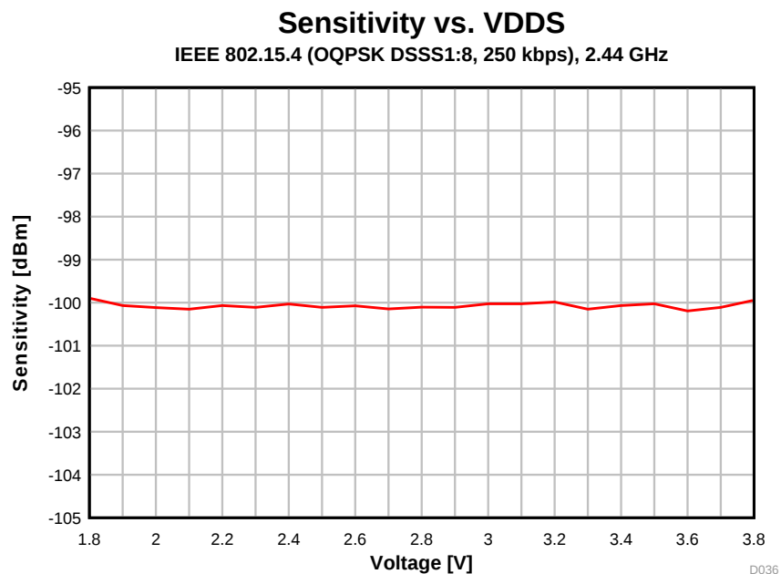
图 5-27. Sensitivity vs. Supply Voltage (VDDS) (250 kbps, 2.44 GHz)
