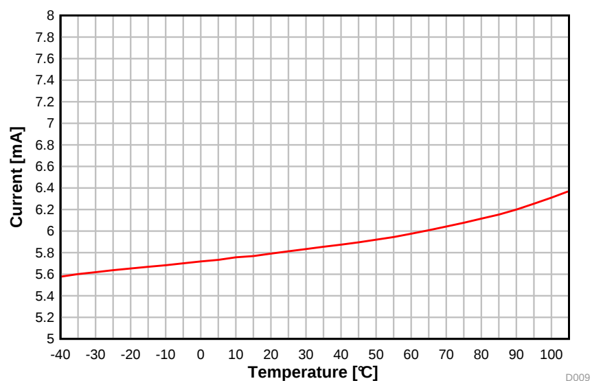
图 5-8. RX Current vs. Temperature (50 kbps, 868.3 MHz, VDD5 = 3.6 V)
