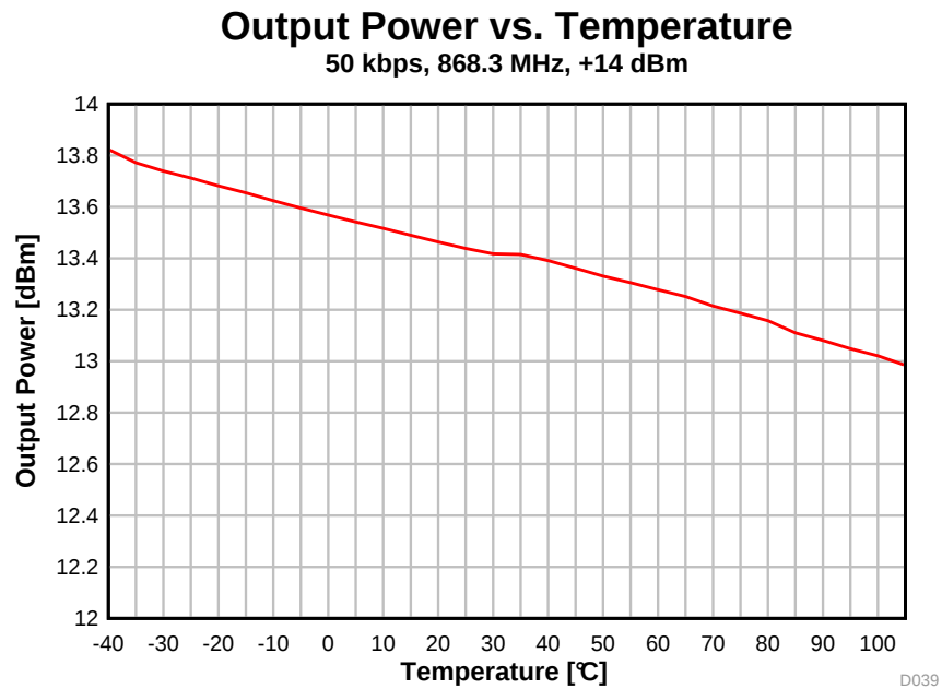
图 5-29. Output Power vs. Temperature (50 kbps, 868.3 MHz)
