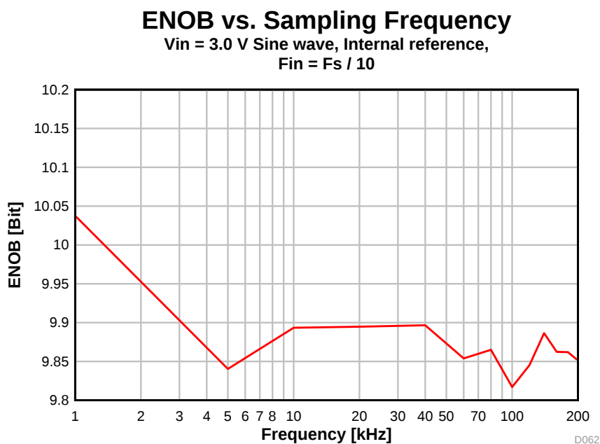
图 5-40. ENOB vs. Sampling Frequency
