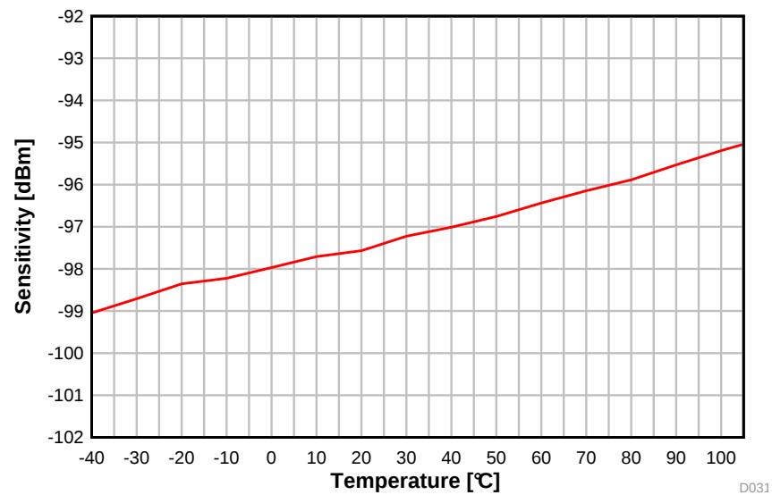
图 5-22. Sensitivity vs. Temperature (BLE 1 Mbps, 2.44 GHz)
