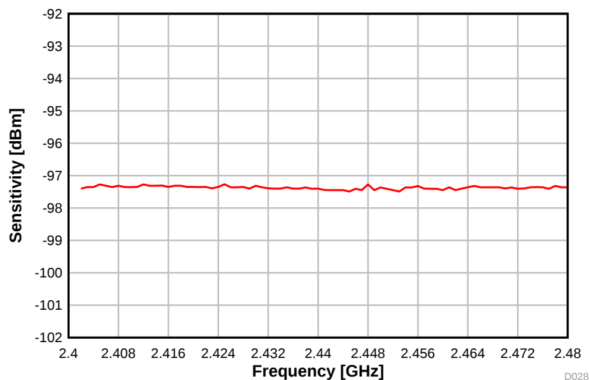
图 5-23. Sensitivity vs. Frequency (BLE 1 Mbps, 2.44 GHz)
