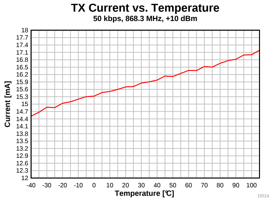
图 5-12. TX Current vs. Temperature (50 kbps, 868.3 MHz)
