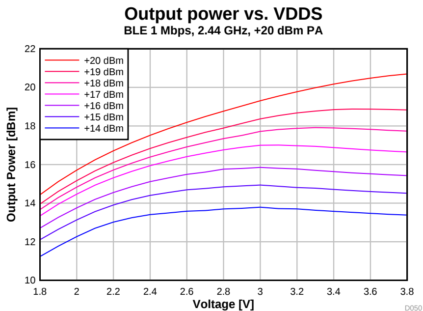
图 5-42. Output Power vs. Supply Voltage (VDD5) (BLE 1 Mbps, 2.44 GHz, +20 dBm PA)
