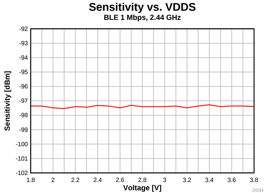
图 5-29. Sensitivity vs. Supply Voltage (VDD5) (BLE 1 Mbps, 2.44 GHz)
