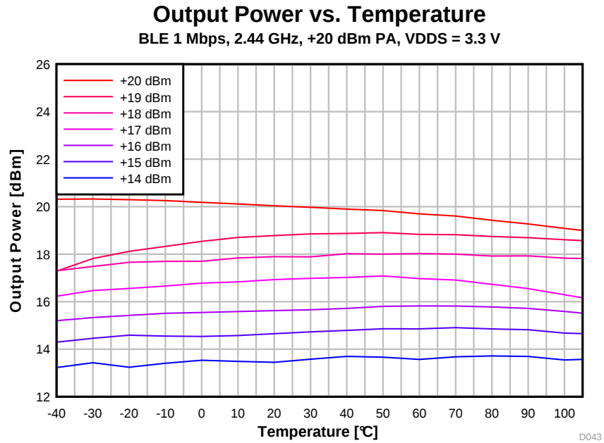
图 5-37. Output Power vs. Temperature (BLE 1 Mbps, 2.44 GHz, +20 dBm PA)
