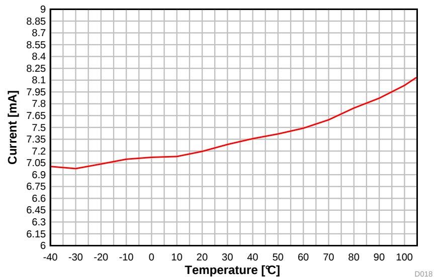
图 5-15. TX Current vs. Temperature (BLE 1 Mbps, 2.44 GHz)
