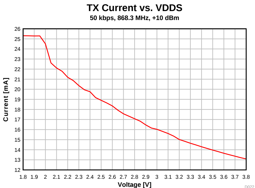
图 5-17. TX Current vs. Supply Voltage (VDD5) (50 kbps, 868.3 MHz)
