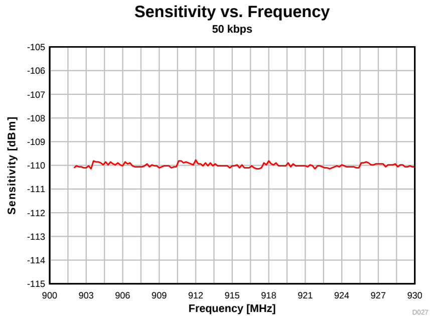
图 5-22. Sensitivity vs. Frequency (50 kbps, 915 MHz)
