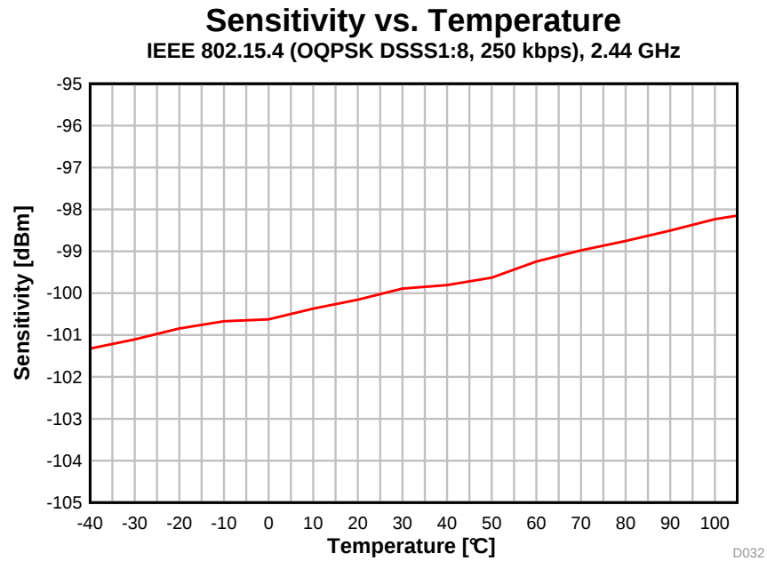
图 5-27. Sensitivity vs. Temperature (250 kbps, 2.44 GHz)
