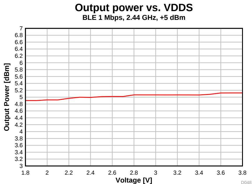
图 5-41. Output Power vs. Supply Voltage (VDD5) (BLE 1 Mbps, 2.44 GHz, +5 dBm)
