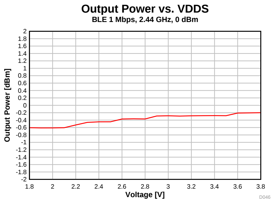
图 5-40. Output Power vs. Supply Voltage (VDDS) (BLE 1 Mbps, 2.44 GHz)
