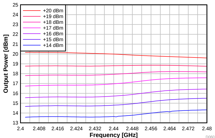
图 5-48. Output Power vs. Frequency (BLE 1 Mbps, 2.44 GHz, +20 dBm PA)
