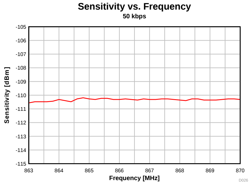
图 5-21. Sensitivity vs. Frequency (50 kbps, 868 MHz)
