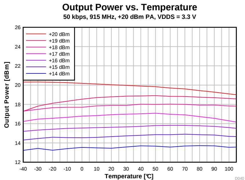
图 5-34. Output Power vs. Temperature (50 kbps, 915 MHz)
