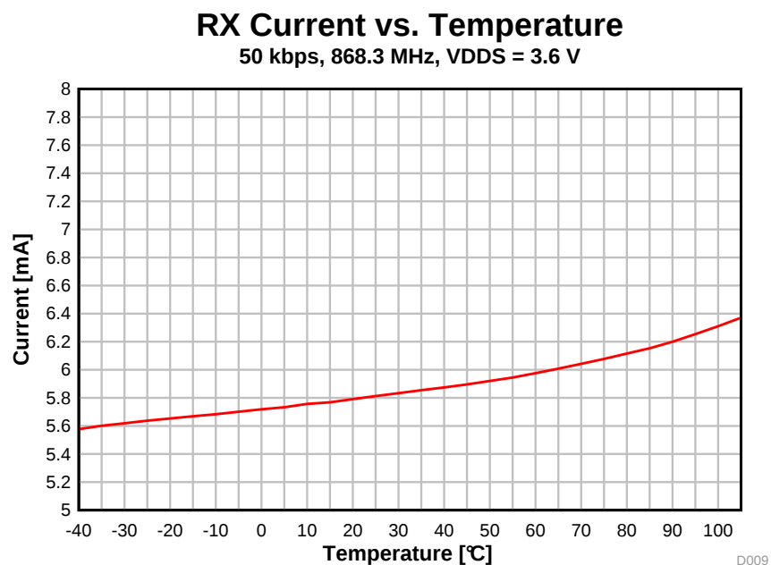
图 5-8. RX Current vs. Temperature (50 kbps, 868.3 MHz, VDD5 = 3.6 V)
