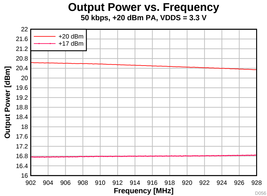
图 5-45. Output Power vs. Frequency (50 kbps, 915 MHz, VDD S = 3.3 V)
