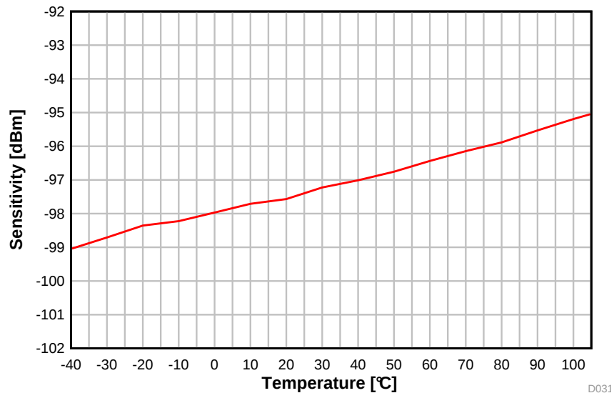
图 5-26. Sensitivity vs. Temperature (BLE 1 Mbps, 2.44 GHz)
