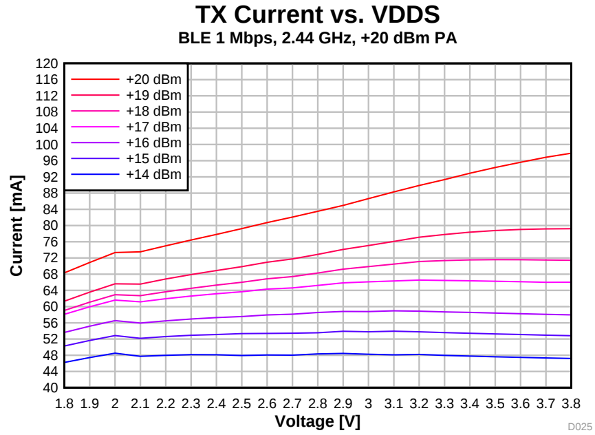
图 5-20. TX Current vs. Supply Voltage (VDD5) (BLE 1 Mbps, 2.44 GHz, +20 dBm PA)
