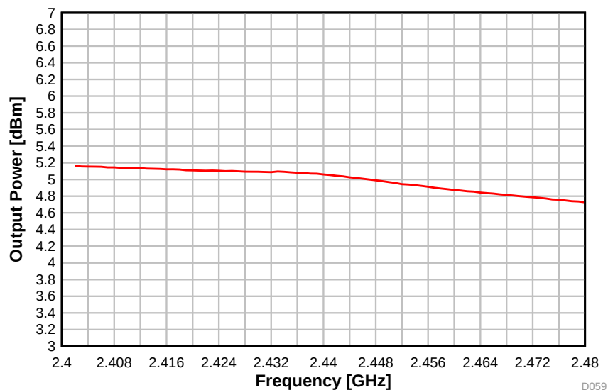
图 5-47. Output Power vs. Frequency (BLE 1 Mbps, 2.44 GHz, +5 dBm)
