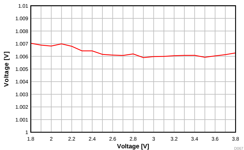
图 5-54. ADC Accuracy vs. Supply Voltage (VDDS)
