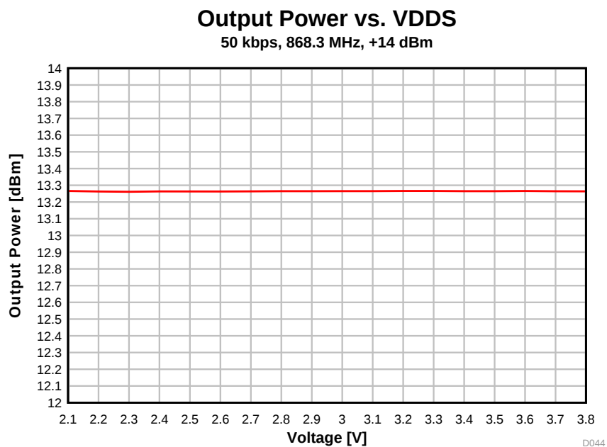
图 5-38. Output Power vs. Supply Voltage (VDD) (50 kbps, 868.3 MHz)
