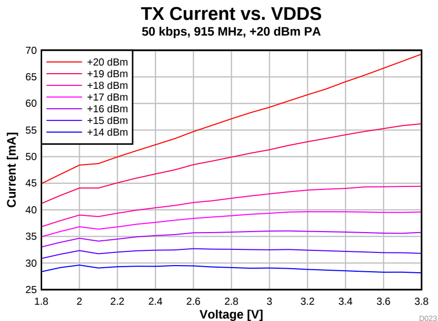
图 5-18. TX Current vs. Supply Voltage (VDDS) (50 kbps, 915 MHz)
