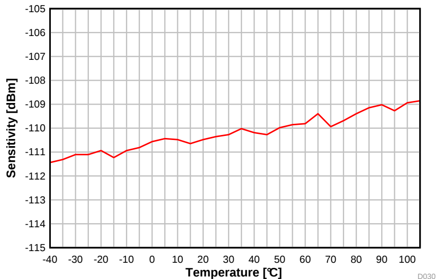
图 5-25. Sensitivity vs. Temperature (50 kbps, 868.3 MHz)
