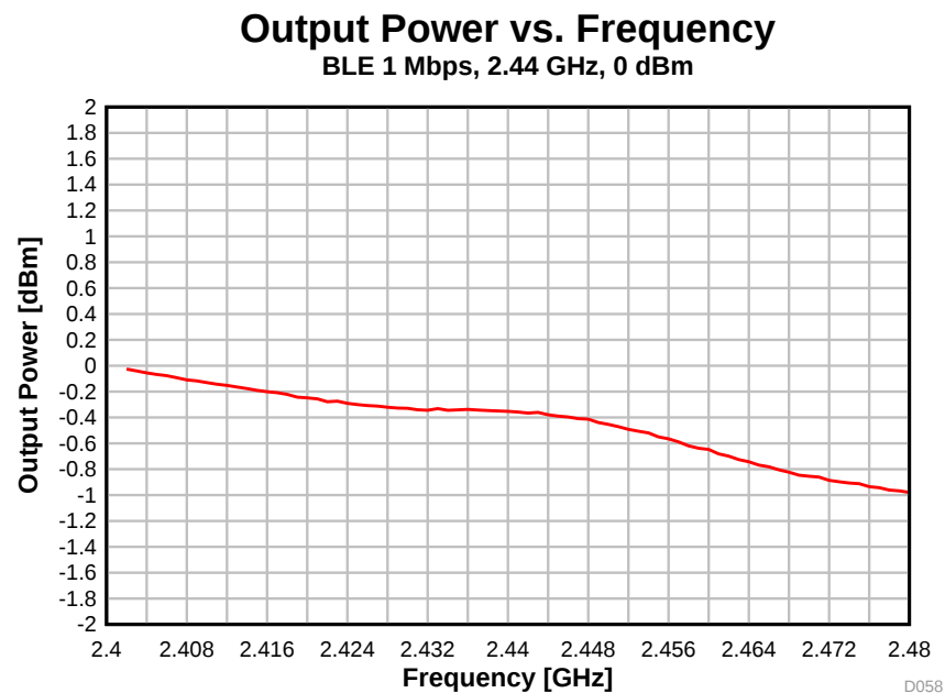
图 5-46. Output Power vs. Frequency (BLE 1 Mbps, 2.44 GHz)
