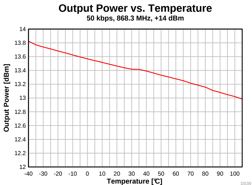
图 5-33. Output Power vs. Temperature (50 kbps, 868.3 MHz)
