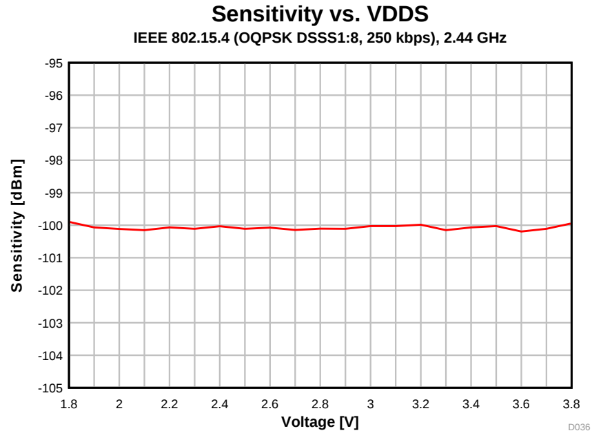
图 5-31. Sensitivity vs. Supply Voltage (VDDS) (250 kbps, 2.44 GHz)
