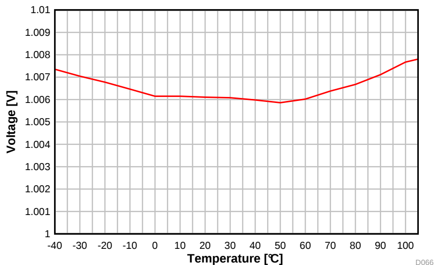
图 5-53. ADC Accuracy vs. Temperature
