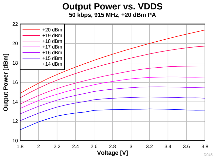
图 5-39. Output Power vs. Supply Voltage (VDDS) (50 kbps, 915 MHz)
