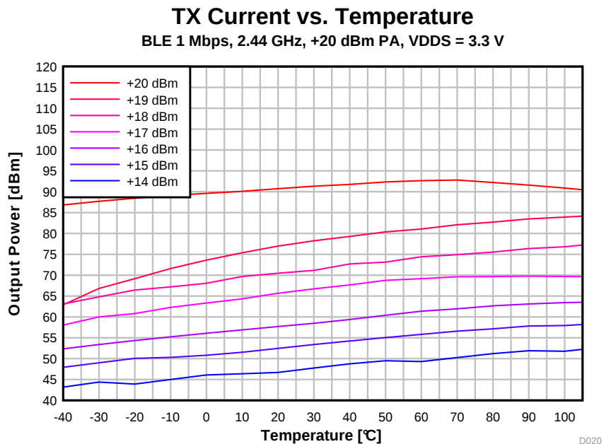
图 5-16. TX Current vs. Temperature (BLE 1 Mbps, 2.44 GHz, VDD5 = 3.3 V)
