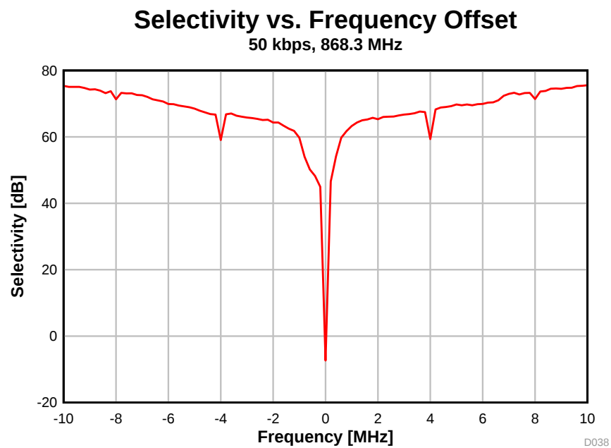
图 5-32. Selectivity vs. Frequency Offset (50 kbps, 868.3 MHz)
