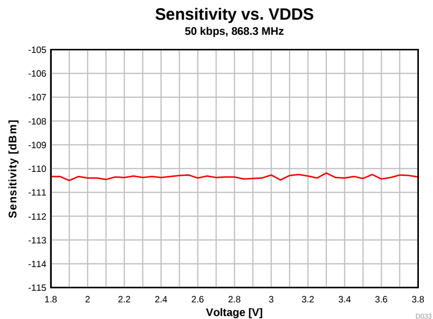
图 5-28. Sensitivity vs. Supply Voltage (VDDS) (50 kbps, 868.3 MHz)
