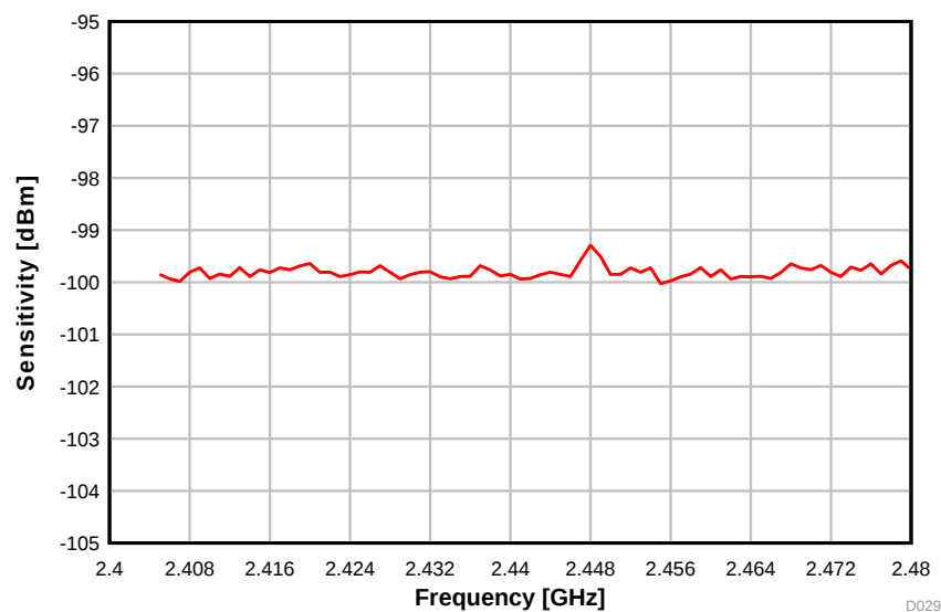
图 5-24. Sensitivity vs. Frequency (250 kbps, 2.44 GHz)
