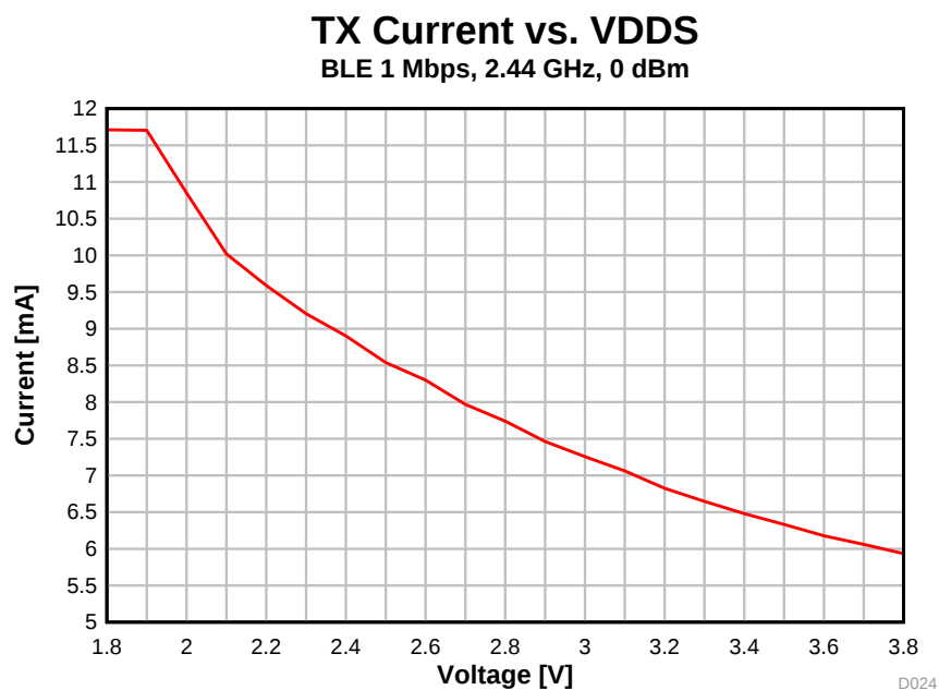
图 5-19. TX Current vs. Supply Voltage (VDDS) (BLE 1 Mbps, 2.44 GHz)
