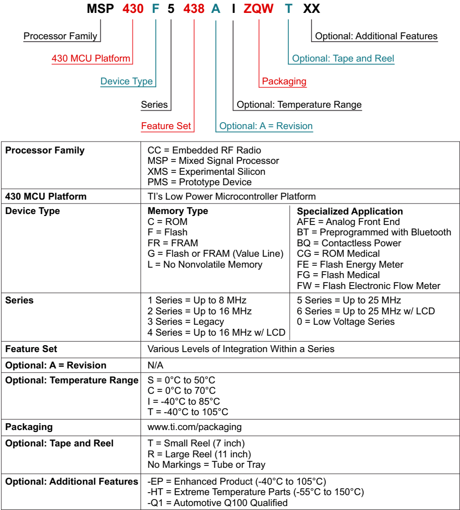
Figure 27. Device Nomenclature
