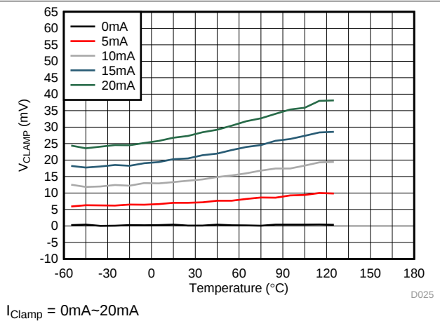
图 24. UCC5310M V_{Clamp} vs Temperature
