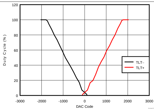
Figure 59. DAC Code vs Duty Cycle for TLT Outputs
