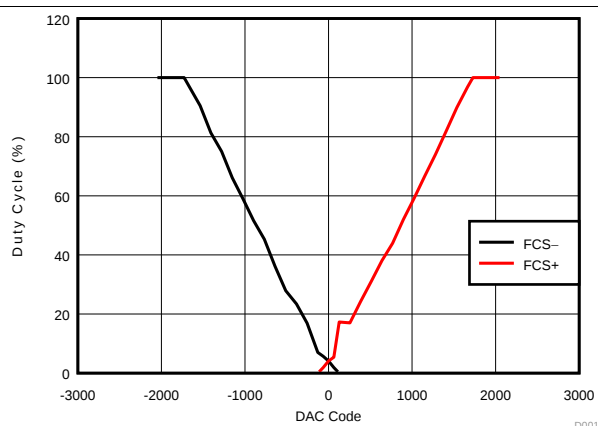
Figure 58. DAC Code vs Duty Cycle for FCS Outputs
