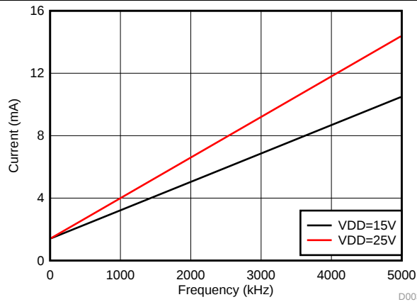
图 4. Per Channel Current Consumption vs. Frequency (No Load, VDD = 15 V or 25 V)
