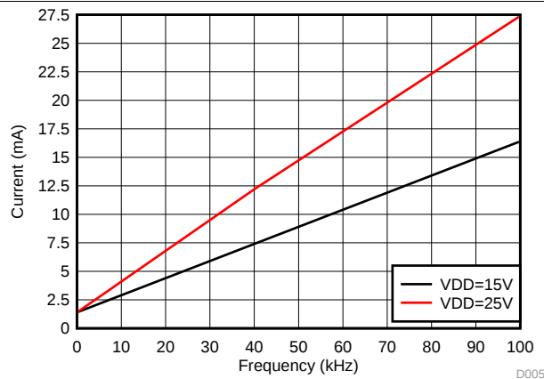
图 4. Per Channel Current Consumption vs. Frequency (No Load, VDD = 15 V or 25 V)
