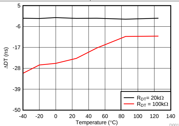
图 25. Dead Time vs. Temperature (with R DT = 20 kΩ and 100 kΩ)
