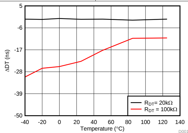
图 25. Dead Time vs. Temperature (with R_{DT} = 20\text{ k}\Omega and 100\text{ k}\Omega )
