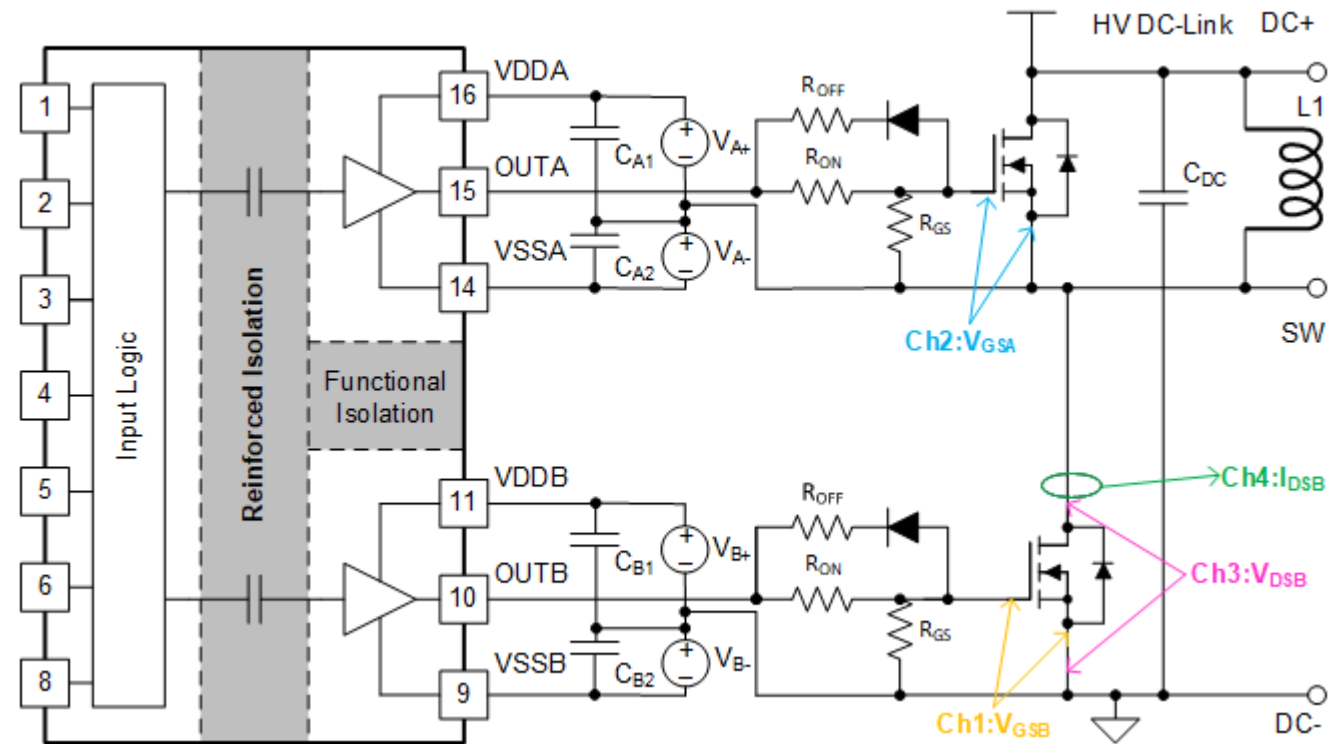
图 42. Bench Test Circuit with SiC MOSFET Switching
