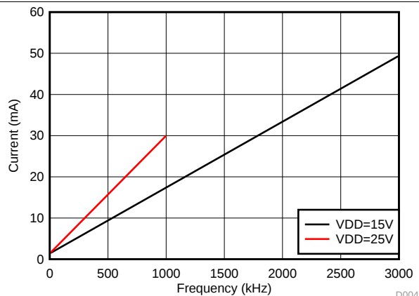
图 5. Per Channel Current Consumption ( I_{VDDA/B} ) vs. Frequency (1-nF Load, VDD = 15 V or 25 V)
