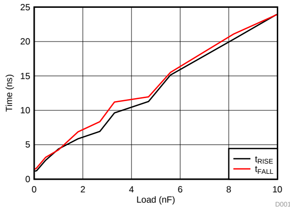
图 10. Rising and Falling Times vs. Load
