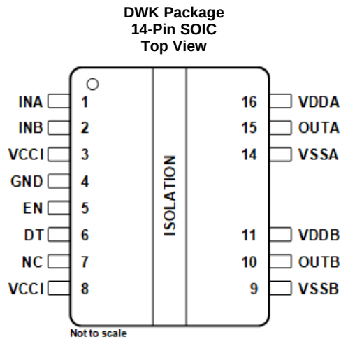
Pin Functions
