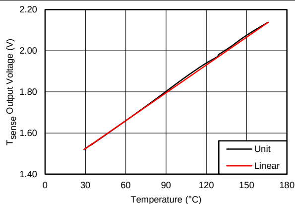
Figure 28. Tsense (Analog Out) Temperature Coefficient: Voltage Plot Example (Typical)
