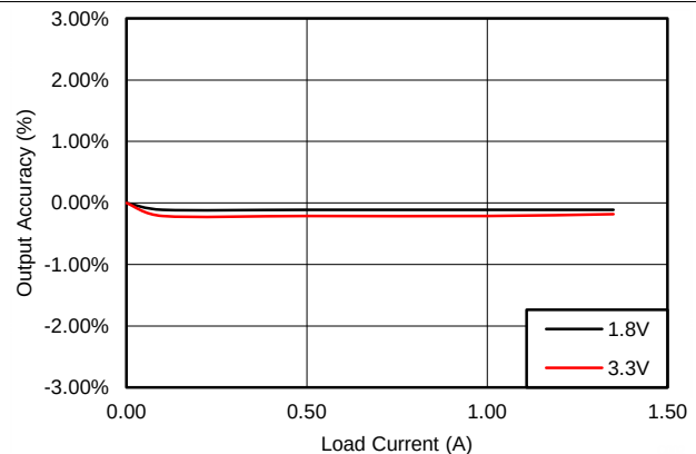
Figure 29. DC-DC Converter - DC Load Regulation Example (Typical)
