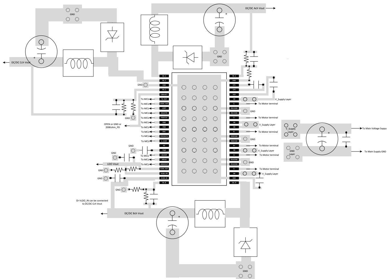
Figure 30. Layout Schematic
