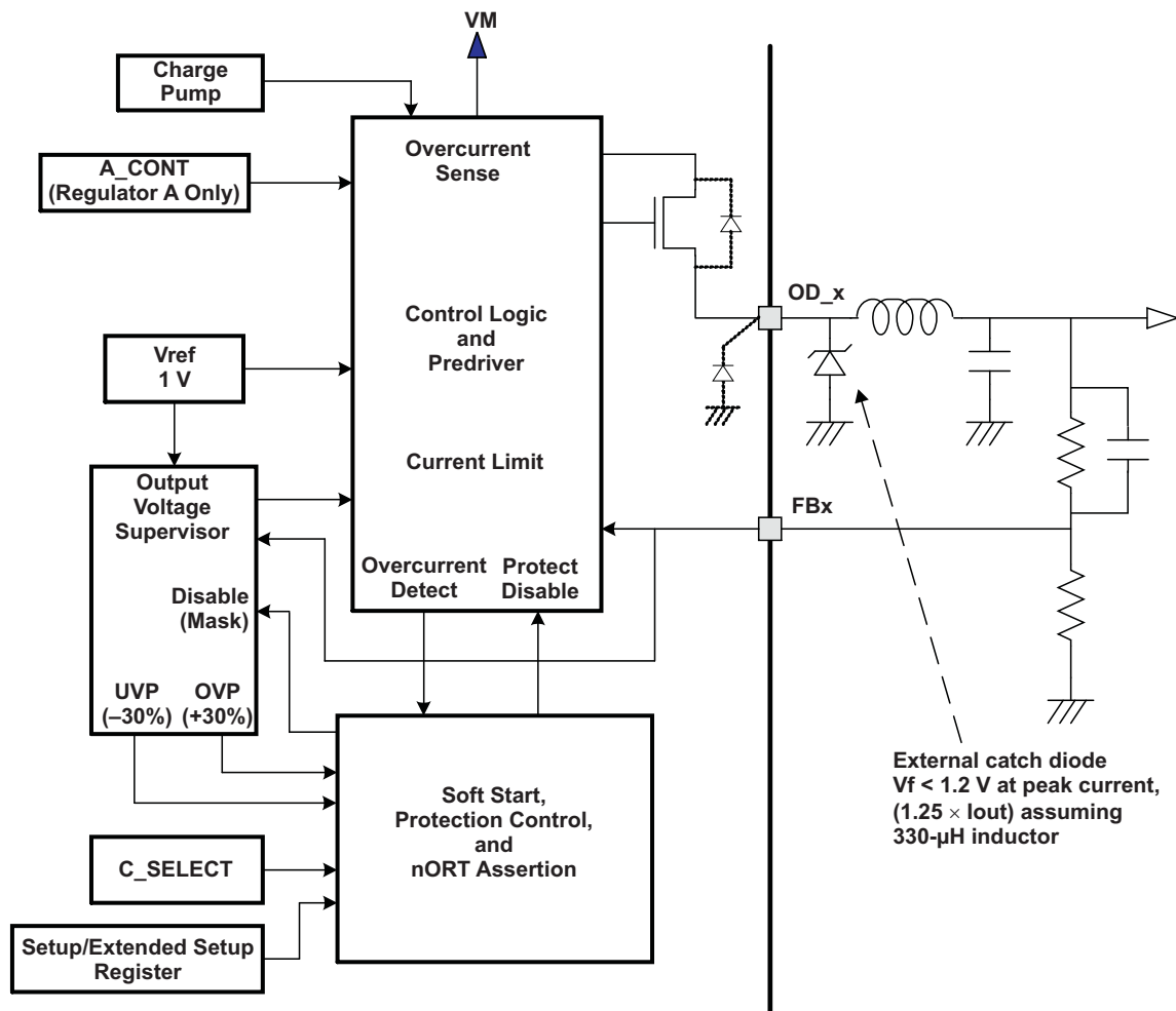
Figure 7. DC-DC Converter
