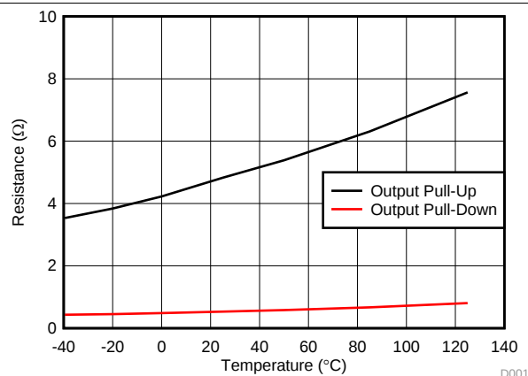
图 11. Output Resistance vs. Temperature
