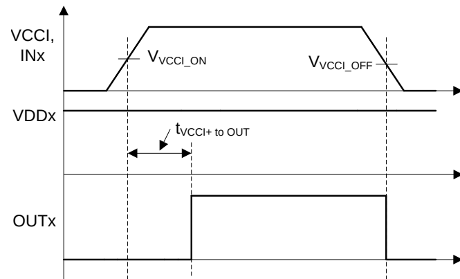
图 31. VCCI Power-up UVLO Delay
