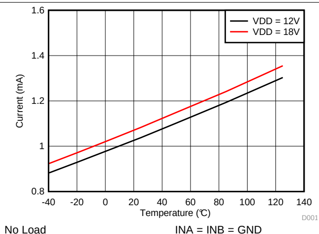
图 6. VDD Per Channel Quiescent Current ( I_{VDDA} , I_{VDDB} )
