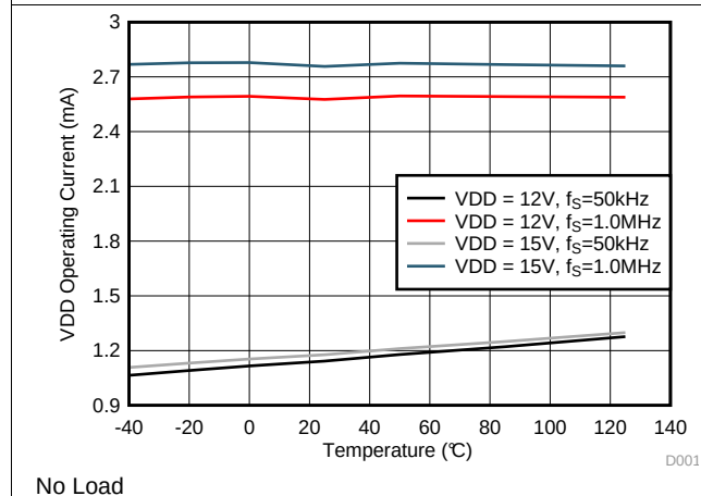
图 7. VDD Per Channel Operating Current - I_{VDDA/B}
