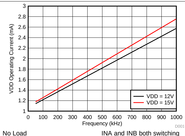
图 8. Per Channel Operating Current ( I_{VDDA/B} ) vs. Frequency
