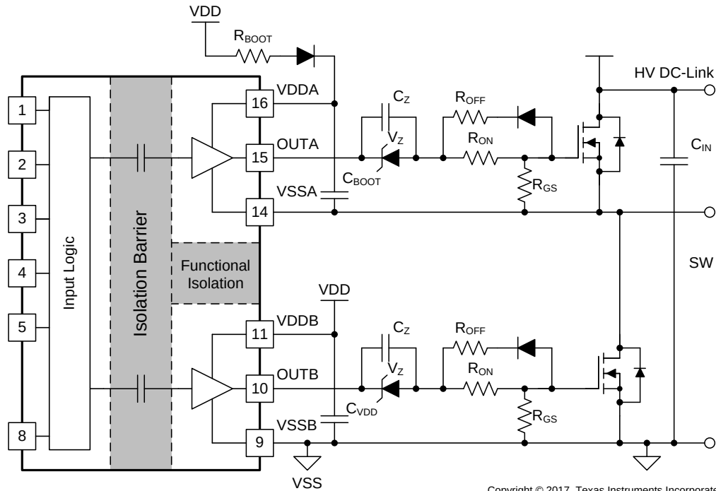
图 39. Negative Bias with Single Power Supply and Zener Diode in Gate Drive Path
