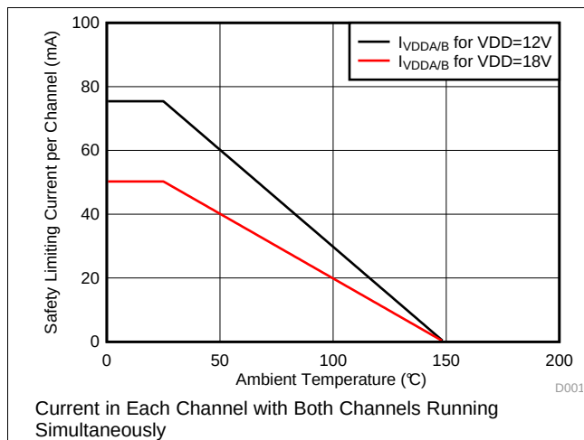
图 1. Thermal Derating Curve for Limiting Current Per VDE
