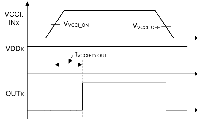
图 30. VCCI Power-up UVLO Delay
