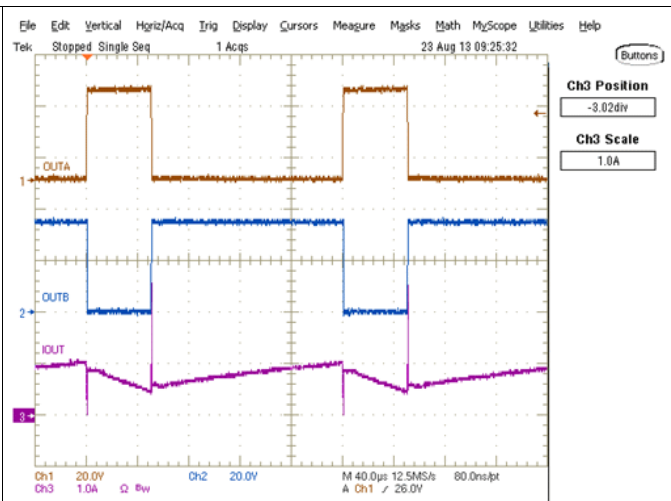
Figure 9. Reverse Drive, Fast Decay
