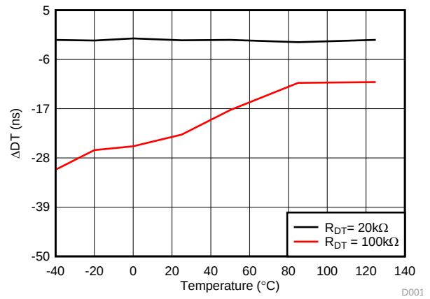
图 23. Dead Time Matching vs. Temperature (with R DT = 20 kΩ and 100 kΩ)
