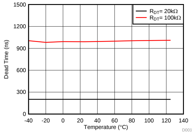
图 22. Dead Time vs. Temperature (with R DT = 20 kΩ and 100 kΩ)
