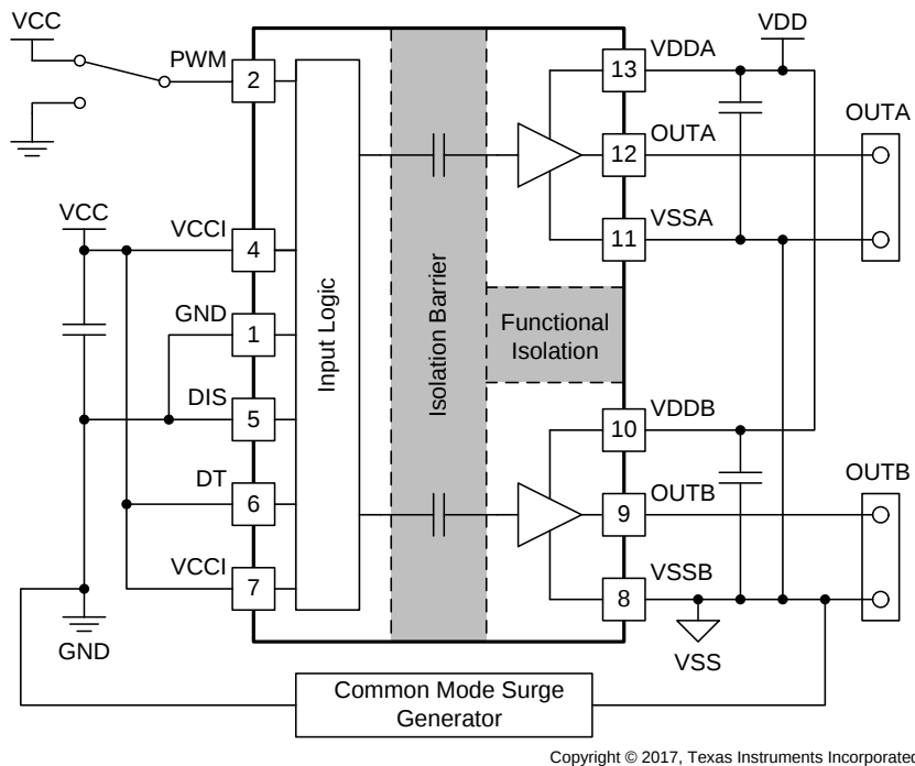
图 30. Simplified CMTI Testing Setup
