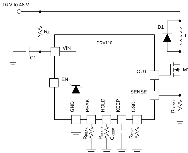
Figure 7. DRV110A-Q1 Powered by a DC Power Source Greater than 15 V
