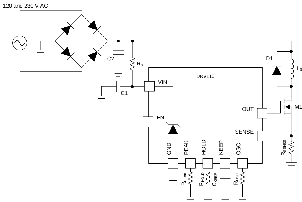
Figure 6. DRV110A-Q1 Powered by a Rectified AC Power Source
