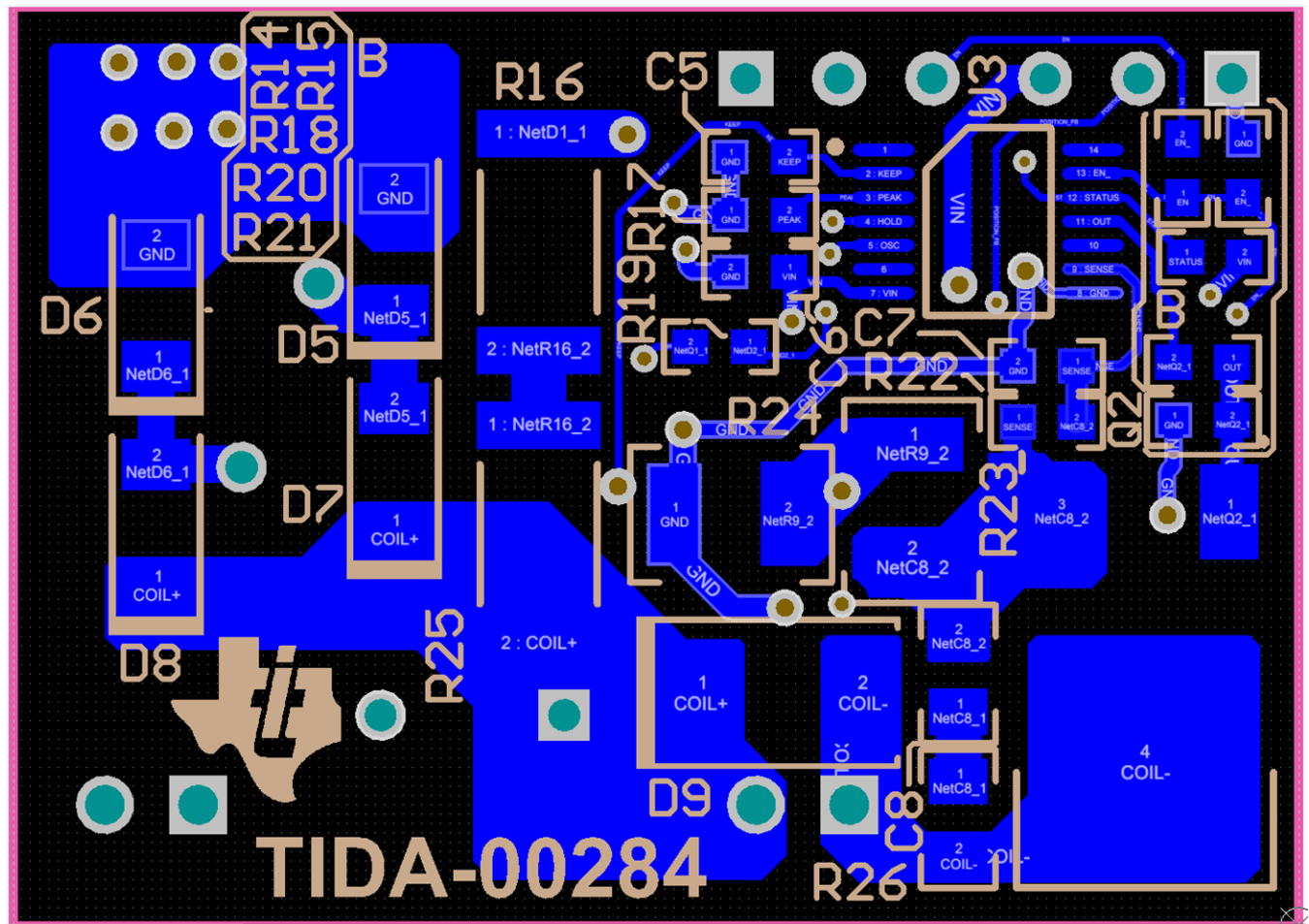
Figure 9. Layout Schematic
