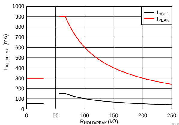
Figure 4. I_{\text{PEAK}} and I_{\text{HOLD}} settings for R_{\text{SENSE}} = 1\Omega
