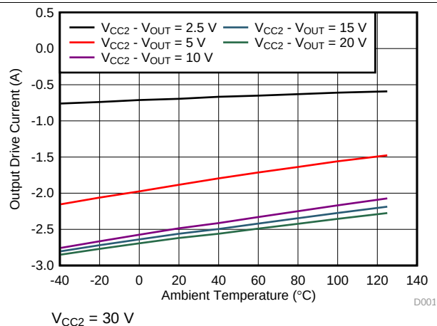
Figure 4. Output High Drive Current vs Temperature
