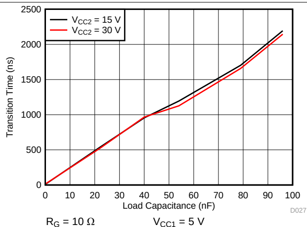
Figure 28. t_f Fall Time vs Load Capacitance
