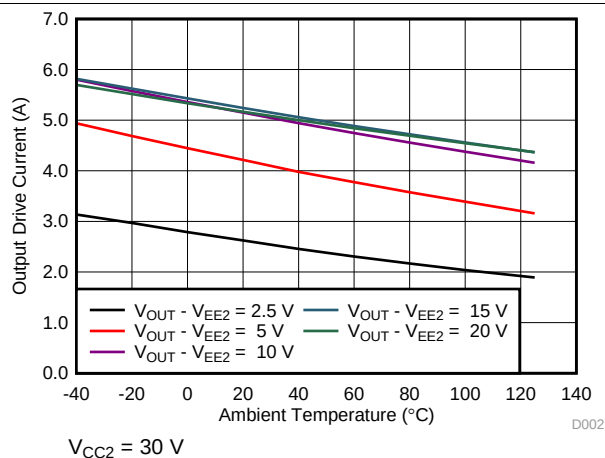
Figure 5. Output Low Drive Current vs Temperature
