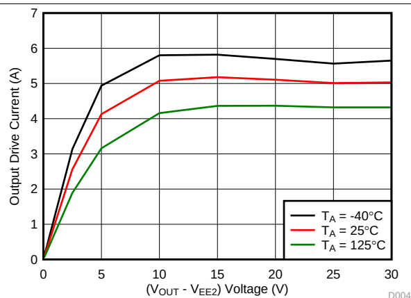
Figure 5. Output Low Drive Current vs Temperature
