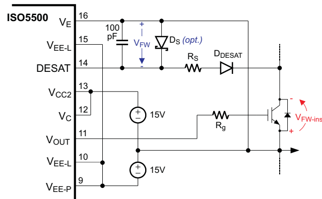
Figure 68. DESAT Pin Protection with Series Resistor and Optional Schottky Diode
