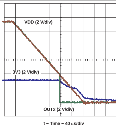
Figure 16. Shut Down Behavior at V_{DD} = 12\text{ V} (Input Tied to 3V3)
