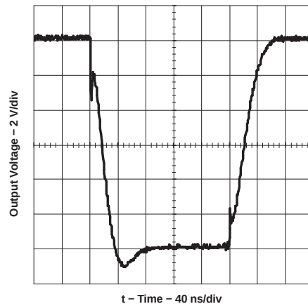
Figure 21. Output Rise and Fall Time ( V_{DD} = 12 V, C_{LOAD} = 10 nF)
