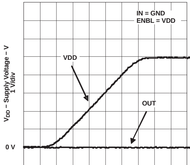
OUTPUT BEHAVIOR VS VDD (NON-INVERTING)
