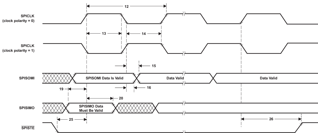
图 5-78. High-Speed SPI Slave Mode External Timing (Clock Phase = 1)
