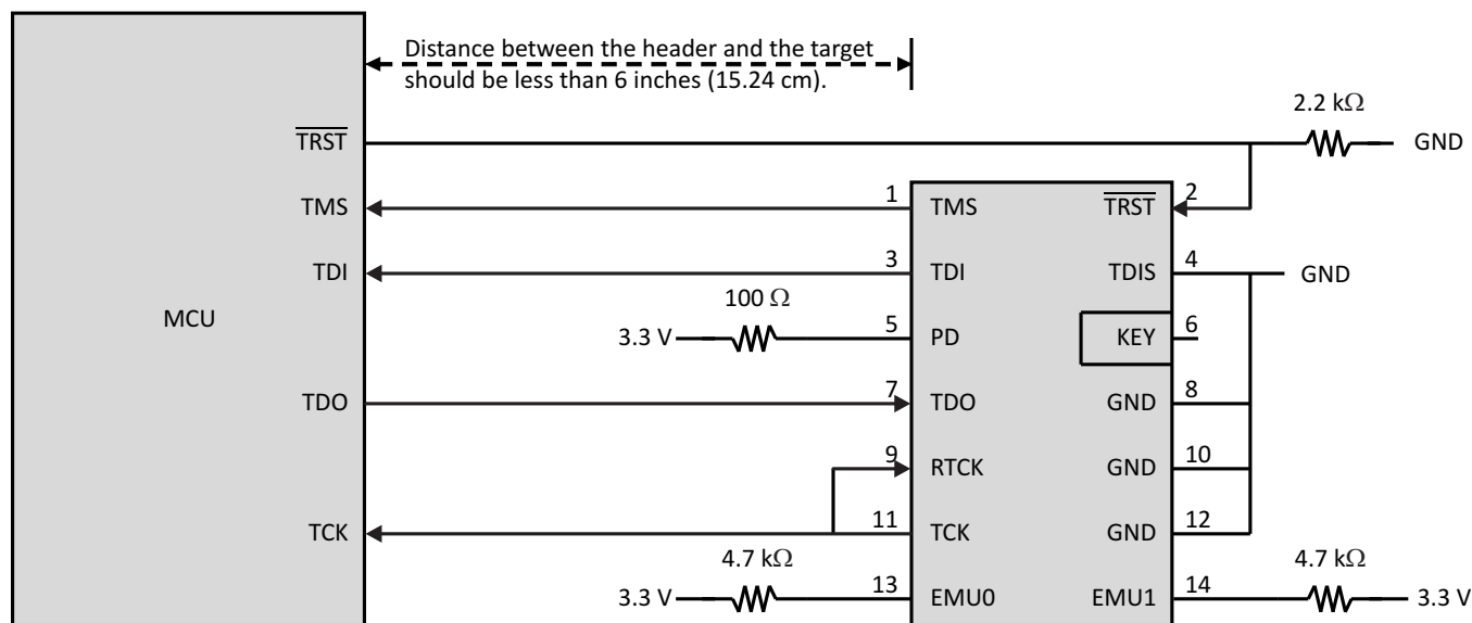
图 5-9. Connecting to the 14-Pin JTAG Header
